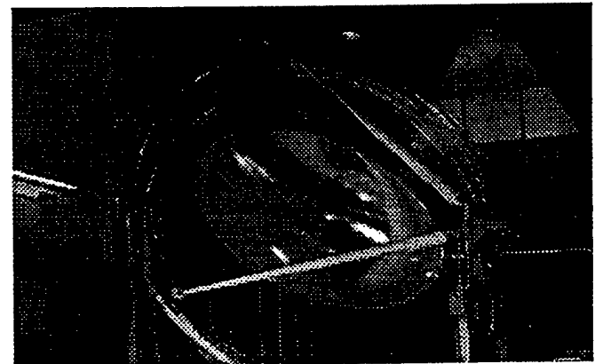
Figure 11. Mandrel and Mandrel Cast Seamless and Goreless Concentrator
