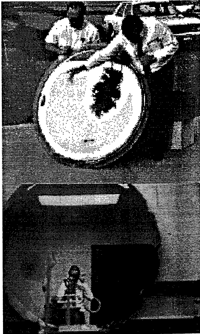
Figure 10. Seamless and Goreless Spin-Cast Reflector
