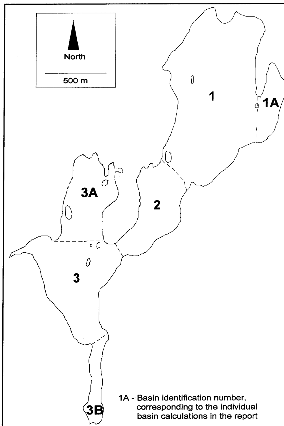
Figure 4. Water basin map of Lake Hortonia, Vermont
