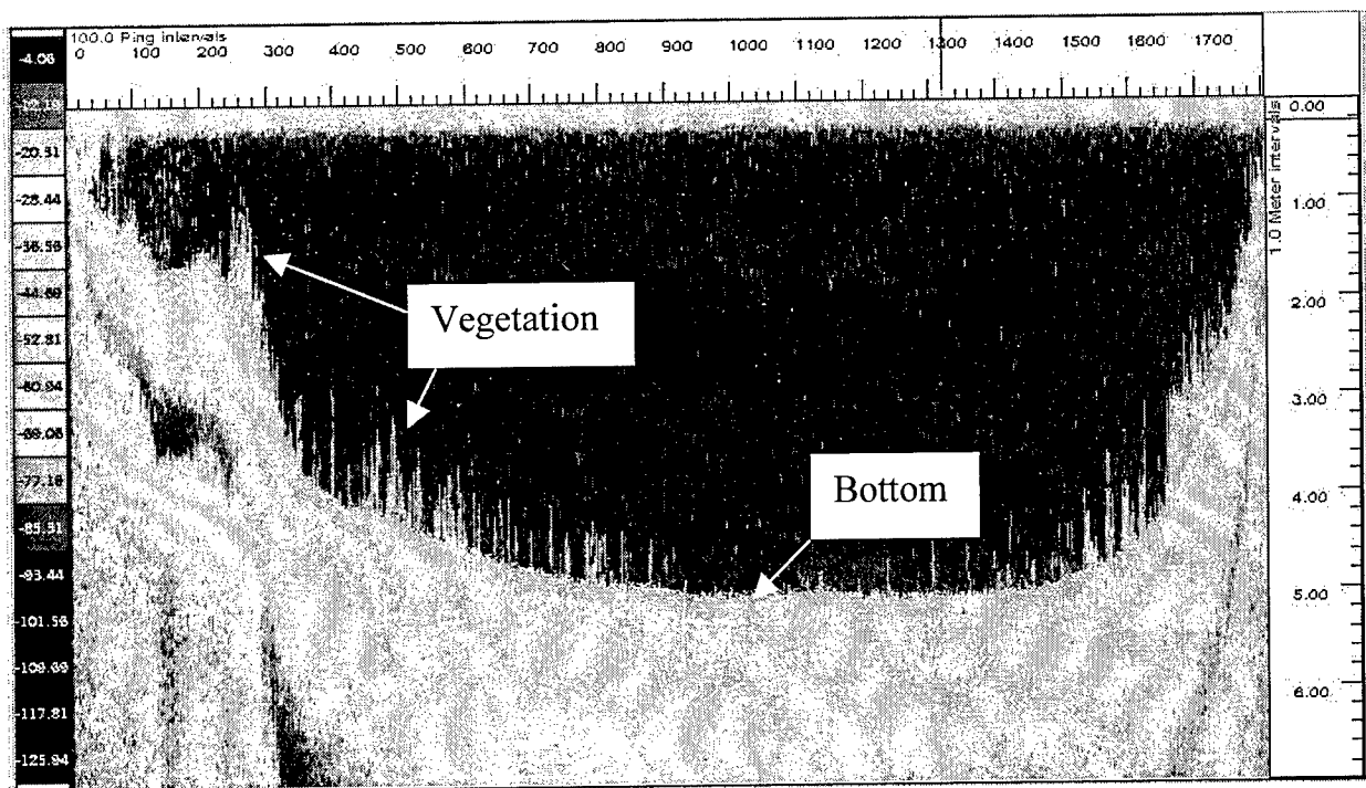
Figure 6. Illustration of hydroacoustic tracing generated by SAVEWS along a transect in Burr Pond during August 2000. Approximate location of the transect in Burr Pond is illustrated in Figure 7
