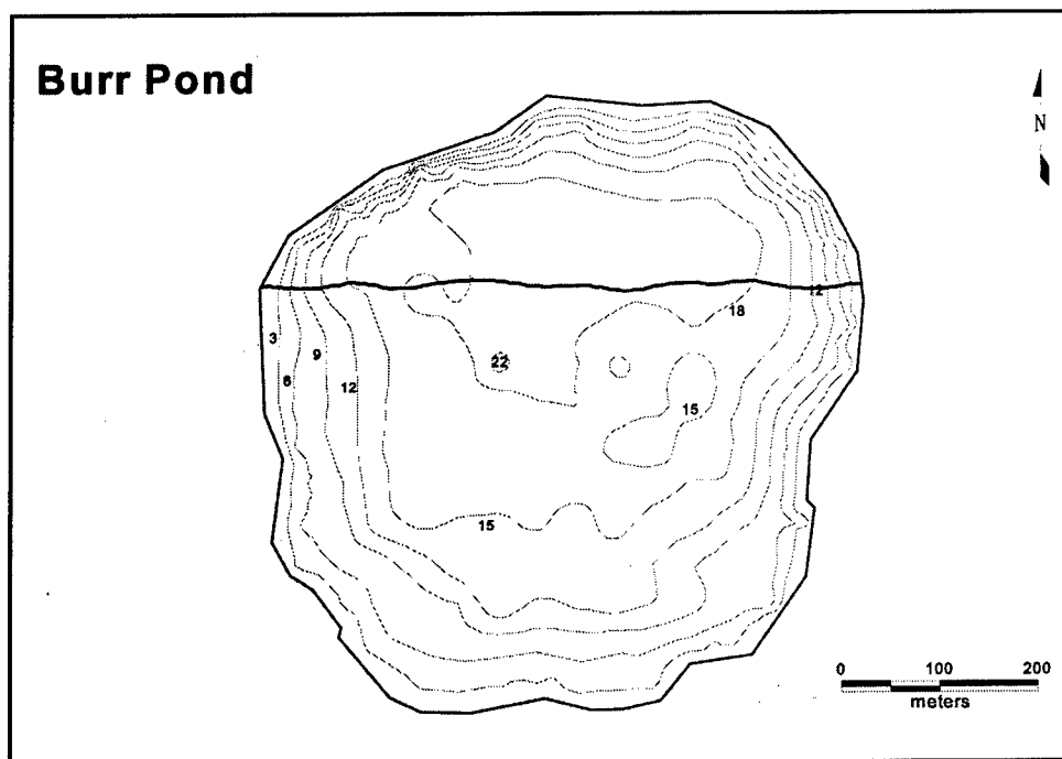
Figure 7. Depth contour map of Burr Pond generated from water depths collected during point-intercept sampling for aquatic plant assessments. The horizontal line indicates the approximate location of west-to-east hydroacoustic survey transect illustrated in Figure 6
