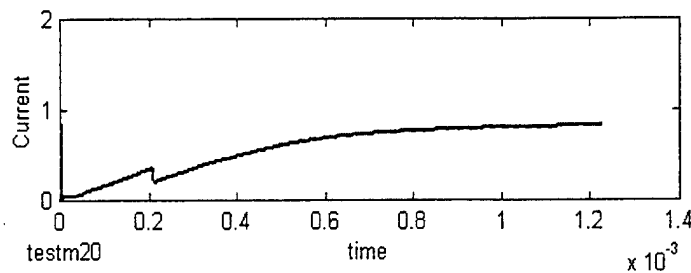
Figure 7 400 V discharge.
