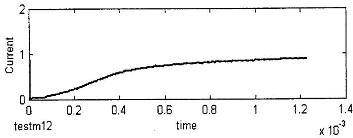
Figure 5 300 V discharge.
