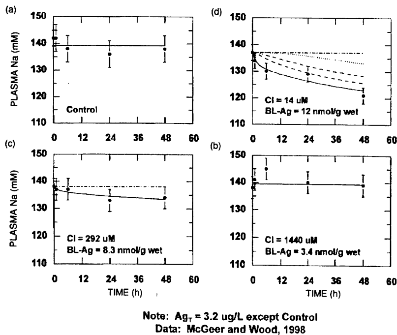
Figure 39. Comparison of rainbow-trout plasma-sodium time-series data (+/- standard error) to model results for control fish ( Ag = 0 ) and fish exposed to 3.2 \mu\text{g/L} of dissolved Ag, as Cl^- varies (McGeer & Wood, 1998).
