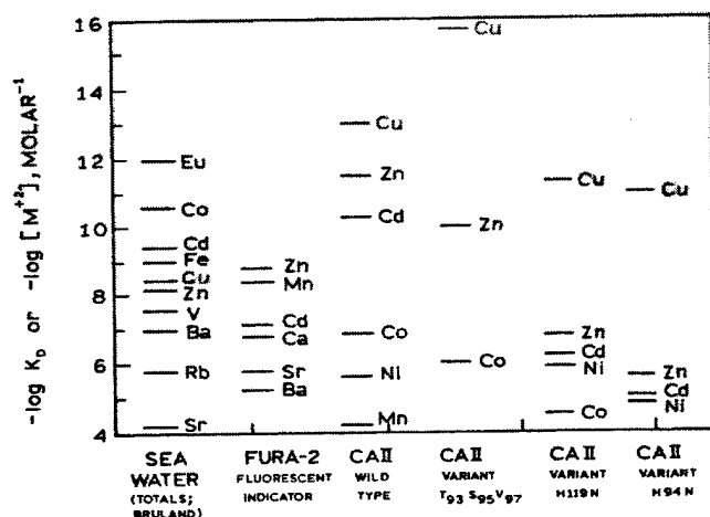
Figure 48. Selectivity of sensor transducers. Affinities for various metal ions are indicated by horizontal lines.
