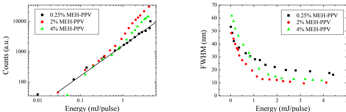
Figure 14. Fluorescence intensity and emission peak FWHM as a function of the pump energy density of MEH-PPV/PS/ZnO (MEH-PPV: 0.25, 2 and 4% w/w, ZnO: 2% w/w) following excitation at 532 nm and 0.0351 \text{ cm}^2 spot size. The solid line denotes slope 1.
