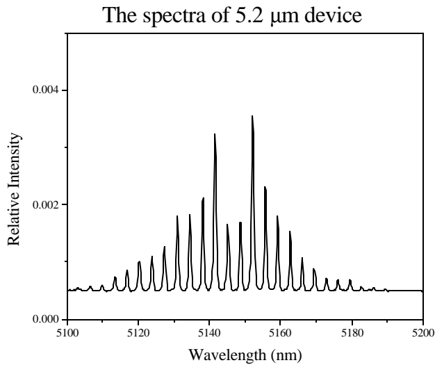
Figure 35. High resolution lasing spectrum at 120 K.
