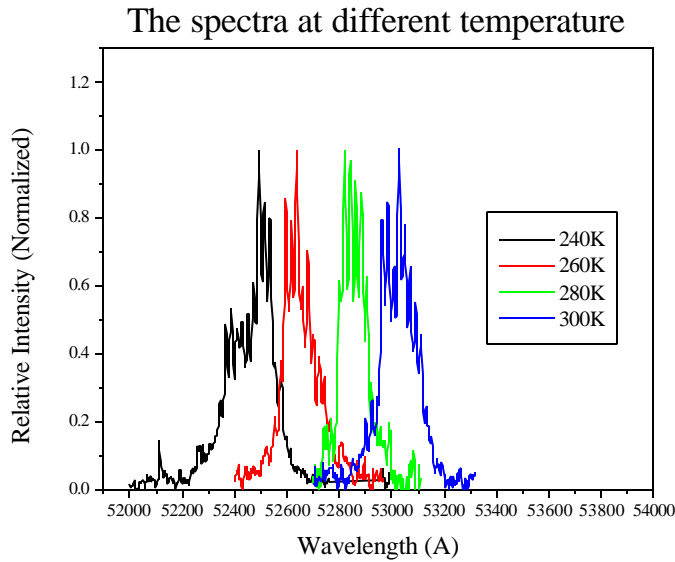
Figure 34. Lasing spectra at different temperatures.
