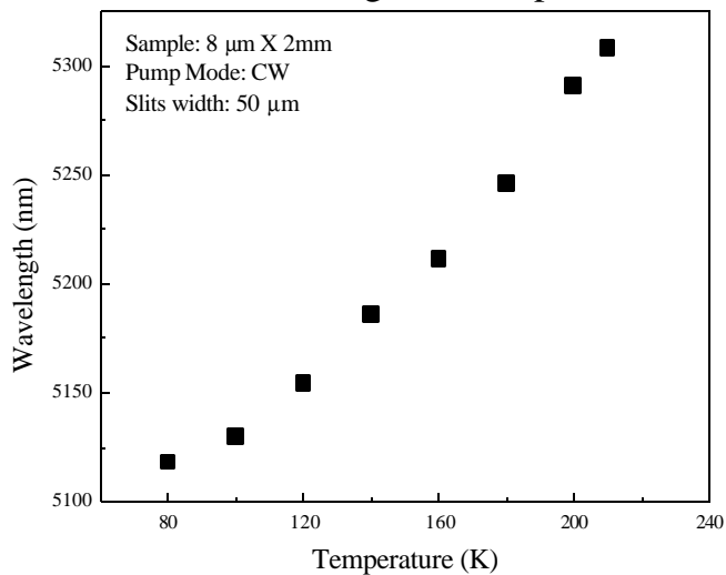
Figure 28. lasing wavelength vs. cryostat temperature at CW mode pumping
