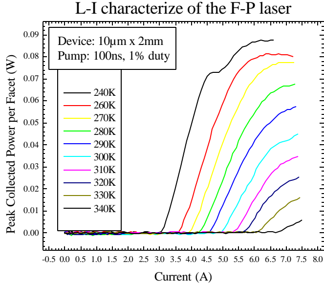
Figure 31. L-I characteristics of the 5.2 mm Type-I QC lasers.
