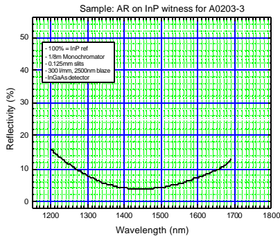
Figure 16. Reflectance spectra of the witness samples of AR coating.
