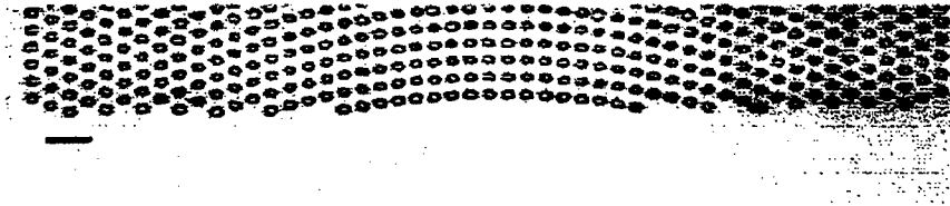
Figure 11. QPM lens, with focal length determined by curvature of the grating. The structure is analogous to a Fresnel lens, since the curved domains have been flattened into a series of convenient thickness sections, with phase resets by an integer number of 2\pi . Fabrication of the lens required use of the improved poling techniques described in section II.1.3.
