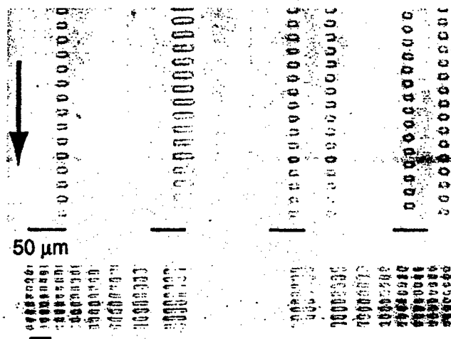
Figure 5. Single and double slit diffraction devices, and a Fresnel lens structure for QPM physical optics demonstrations. The arrow indicates propagation direction; bar represents 50- \mu\text{m} . Domains are revealed by etching. Use of these structures for nonlinear physical optics is discussed in section II.2.3.
