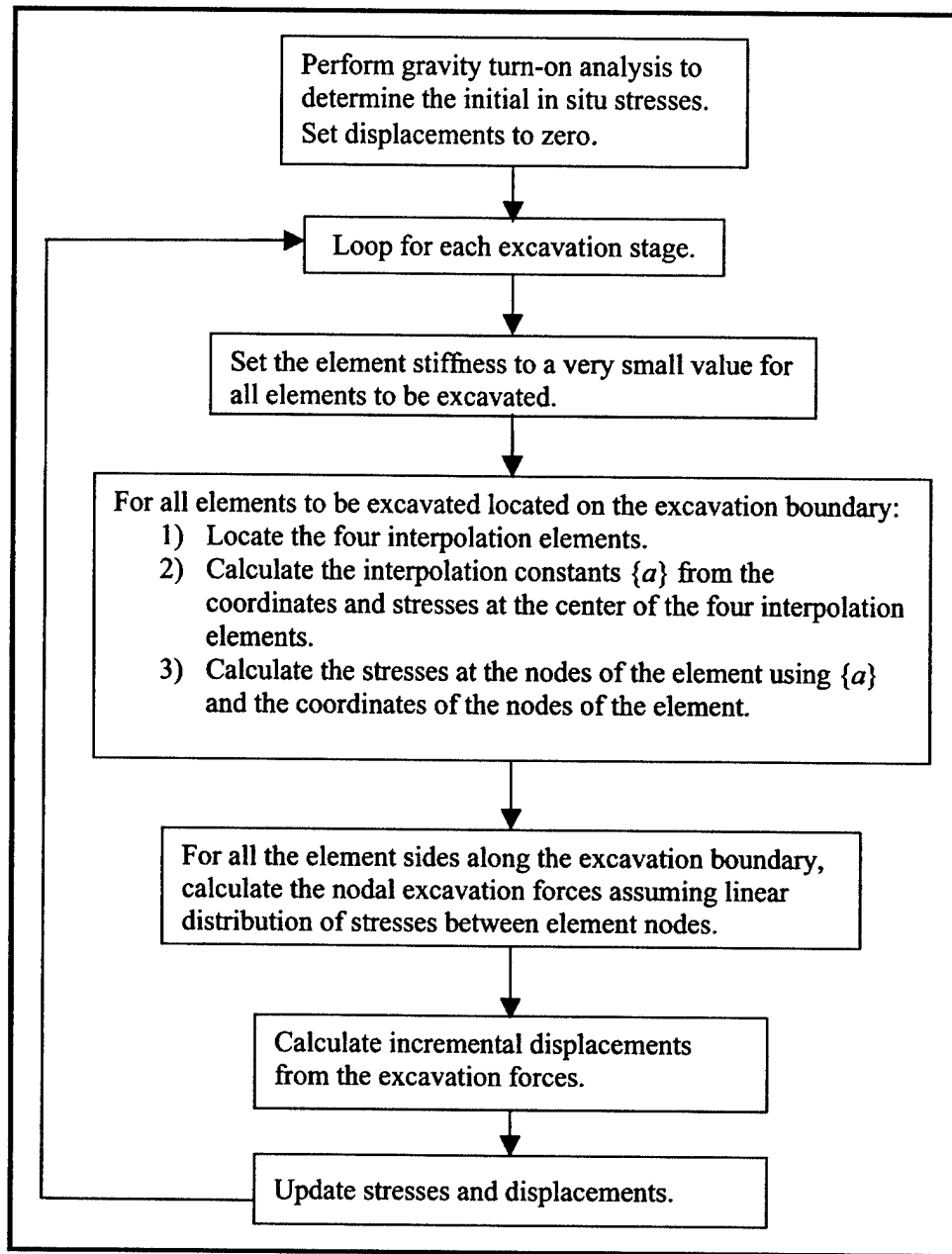
Figure 2.6. Flowchart for excavation modeling using the Clough and Duncan procedure
