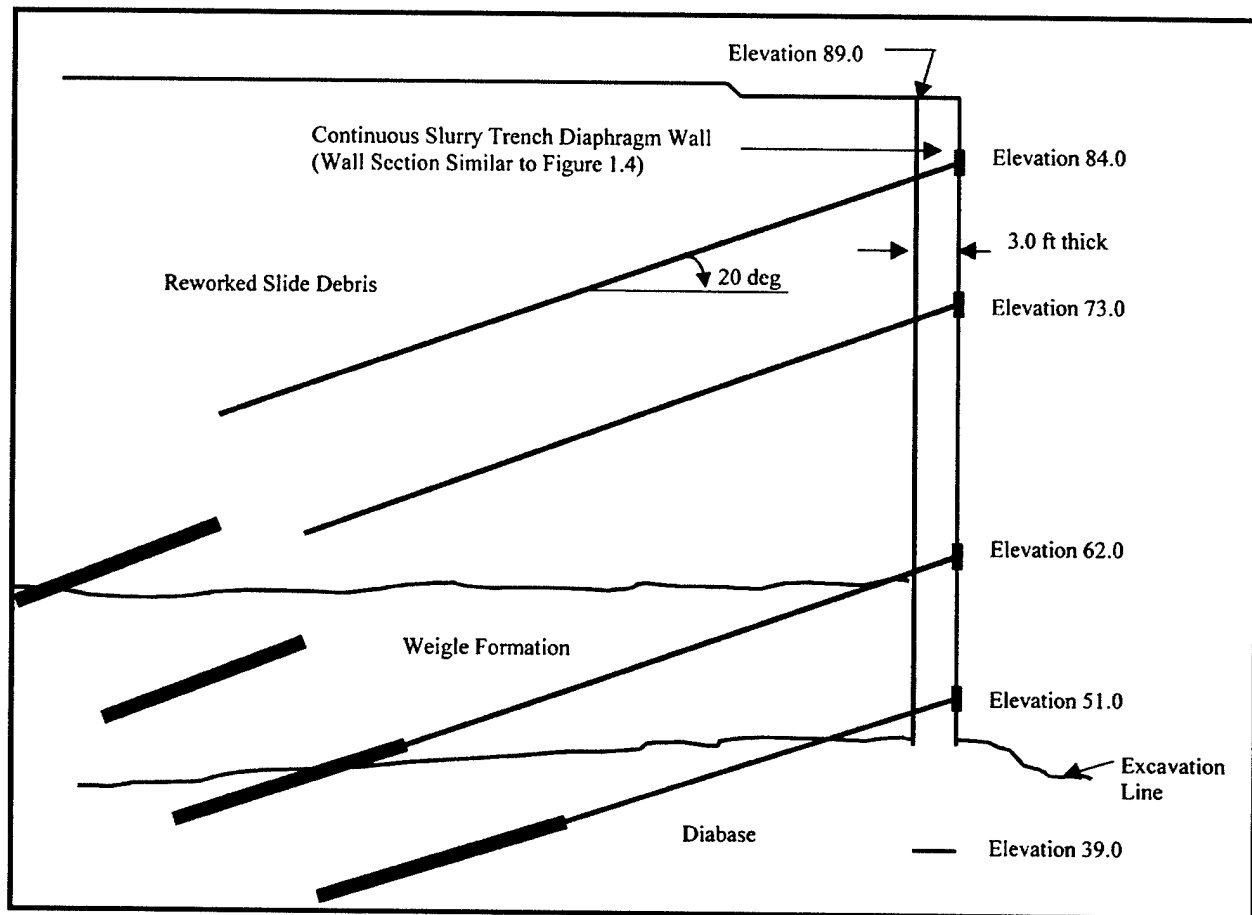
Figure 1.5. Bonneville navigation lock, temporary tieback wall—vertical section (from Strom and Ebeling 2001)
