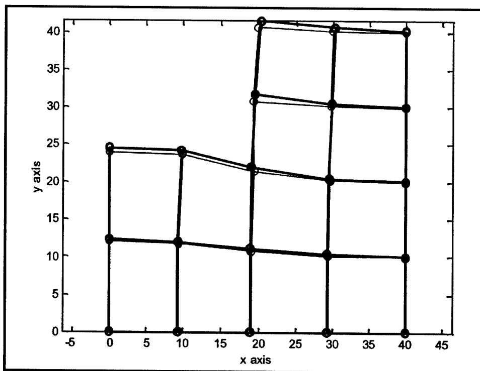
Figure 4.7. Comparison of the results of a single-stage (thin lines) and a two-stage (thick lines) excavation using the Clough and Duncan procedure (deformations magnified 10x)
