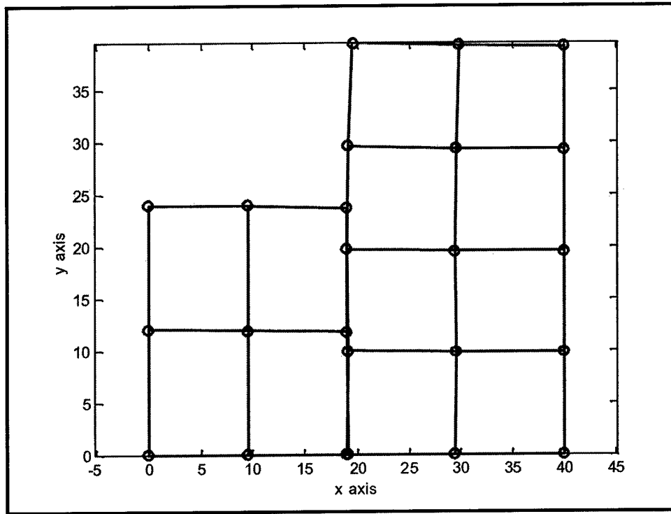
Figure 4.16. Deformed mesh after excavation with K_s = 1 \cdot 10^2 lb/ft (deformations magnified 10x)
