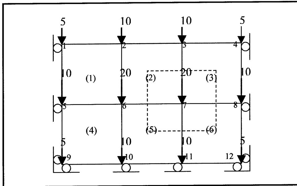
Figure 2.9. Nodal loads from self-weight (forces shown are in kilonewtons)
