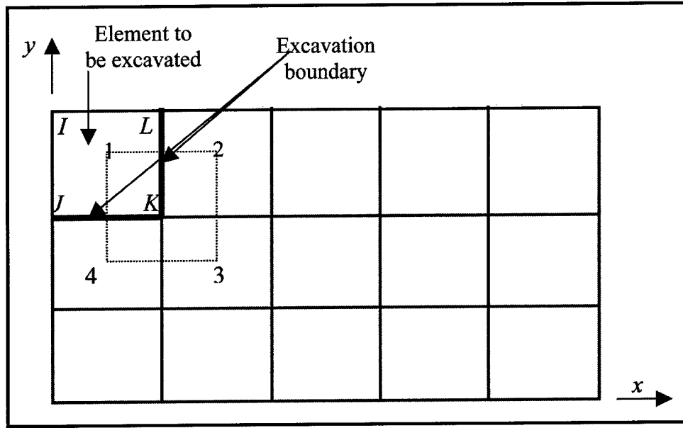
Figure 2.4. Interpolation procedures used to determine the stresses along the excavation boundaries. For the Dunlop, Duncan, and Seed (1968) procedure, stresses along K-L are calculated from the stresses of Elements 1 and 2, and stresses along J-K are calculated from the stresses of Elements 1 and 4. For the Clough and Duncan (1969) procedure, stresses at the nodal points J, K, and L are interpolated from the stresses in the centers of the Elements 1, 2, 3, and 4. Elements 2, 3, and 4 adjacent to the excavated Element 1 are called interpolation elements
