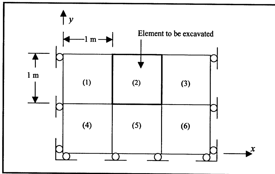
Figure 2.8. Excavation of a single element
