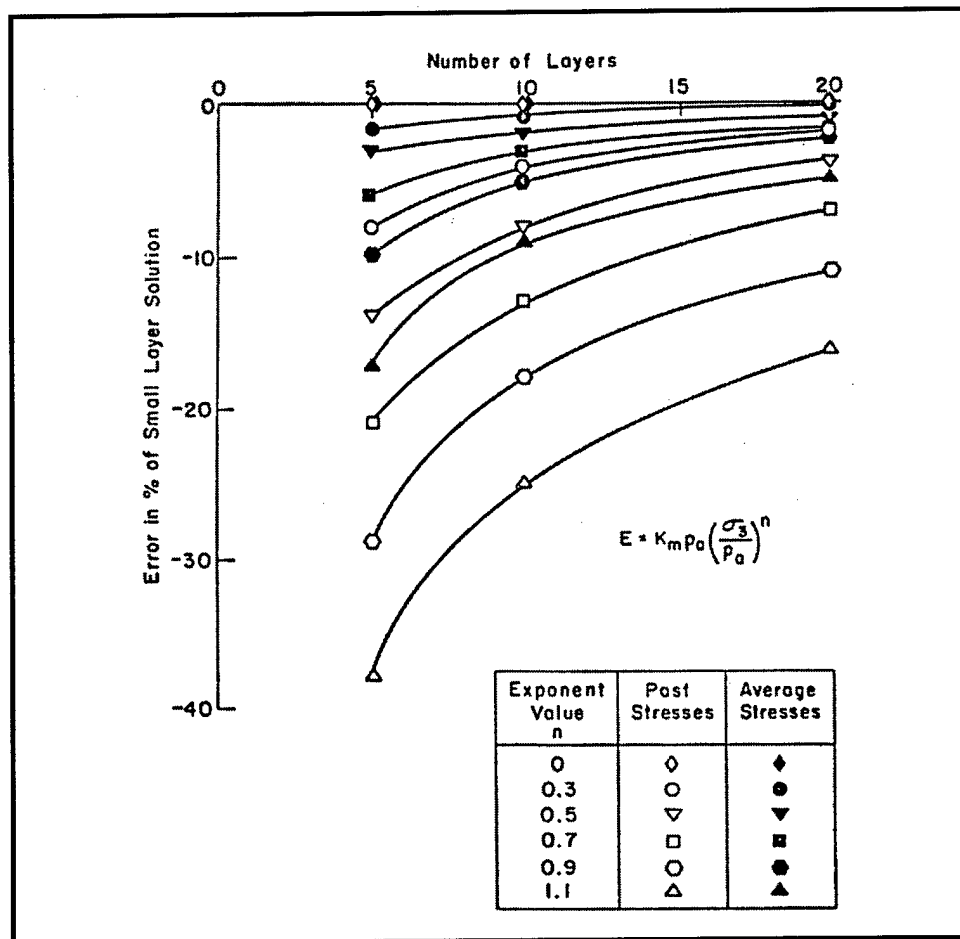
Figure 3.1. Values of errors in simulation of small layer one-dimensional excavation for different values of n (Clough and Duncan 1969)
