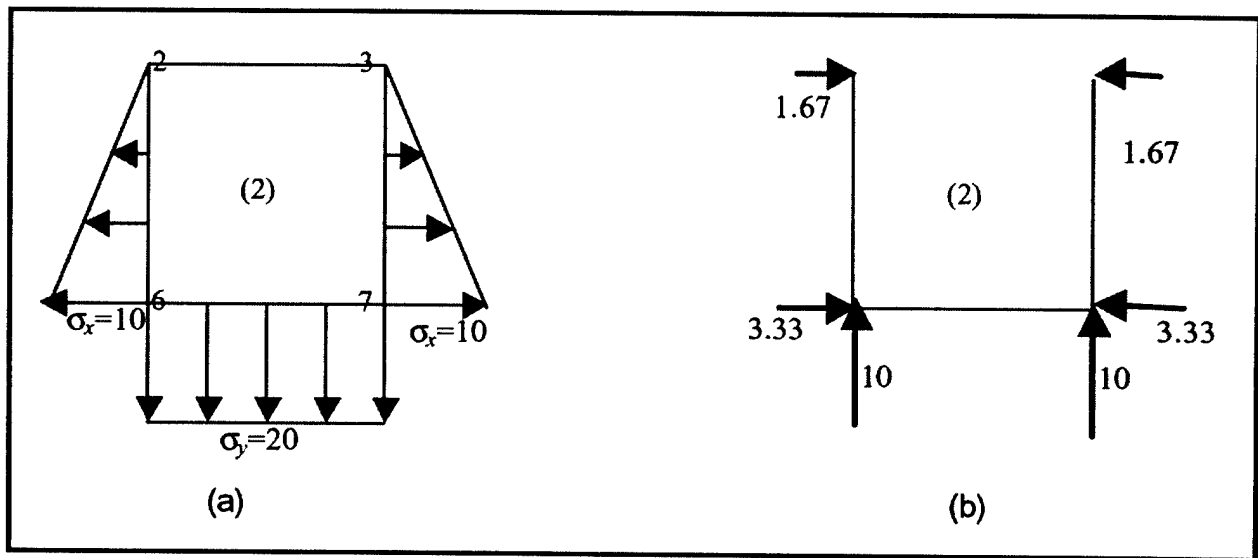
Figure 4.8. Interpolated stresses at element edges (a) and equivalent nodal forces (b) along the excavation boundaries from Element 2, calculated from the Clough and Duncan procedure (stresses are in kilopascals, forces are in kilonewtons)
