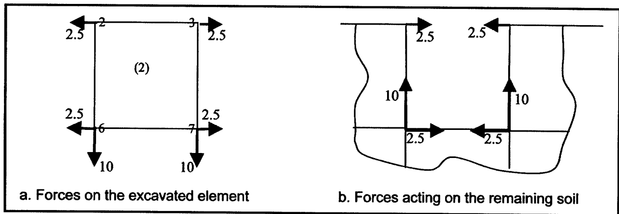
Figure 3.9. Excavation forces along the excavation boundaries (forces are in kilonewtons)
