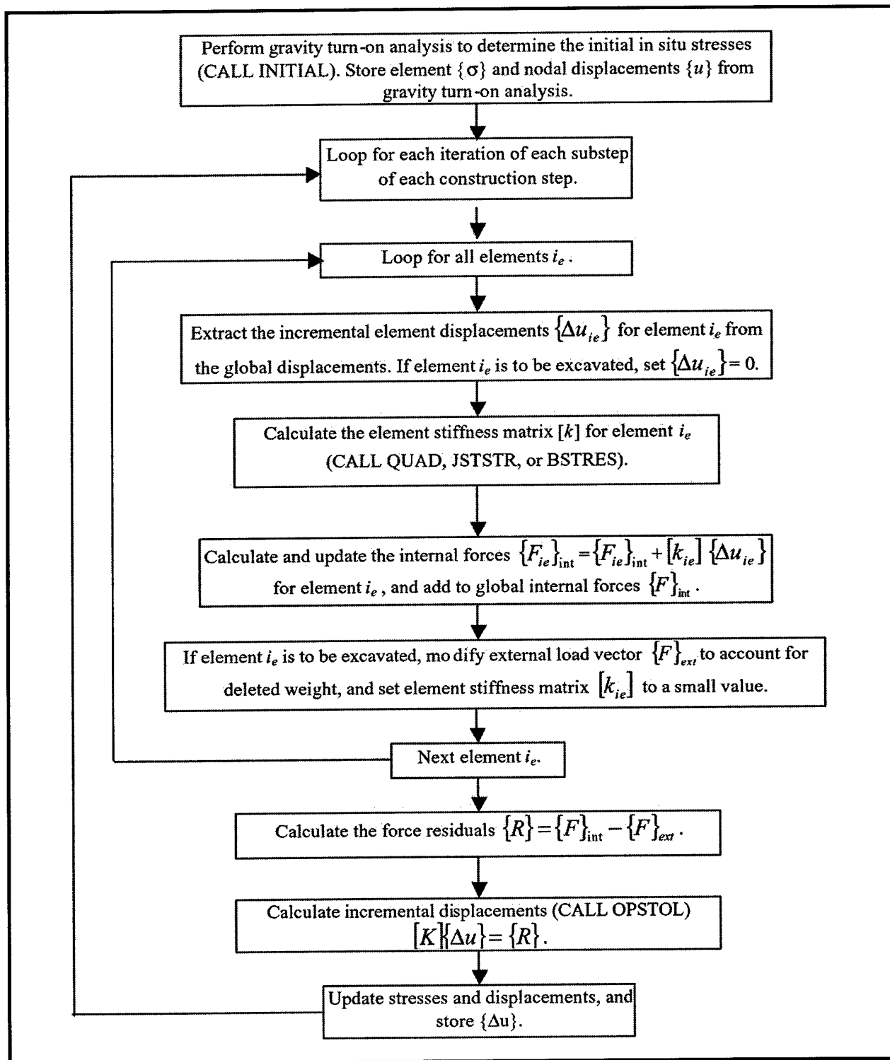
Figure 4.19. Flowchart for implementing the method of force residuals in SOILSTRUCT-ALPHA using incremental element displacements in calculating internal element forces
