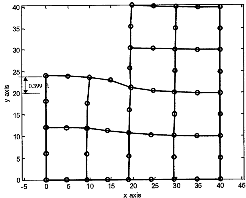
b. Deformed mesh after the second stage of a two-stage excavation
