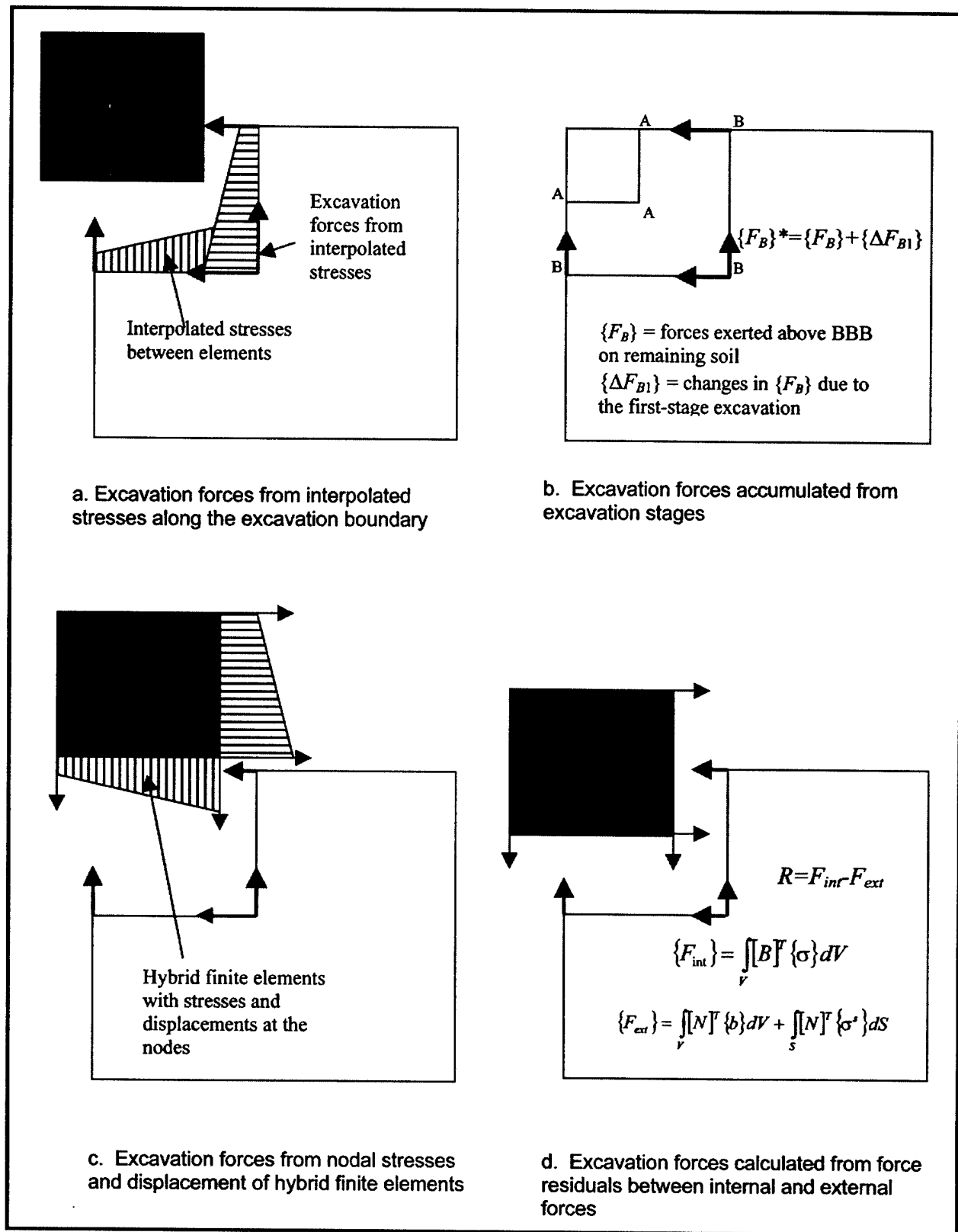
Figure 3.2. Excavation forces
