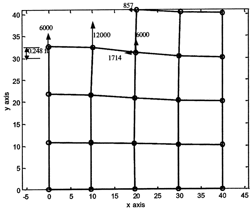
a. Deformed mesh after the first stage of a two-stage excavation
