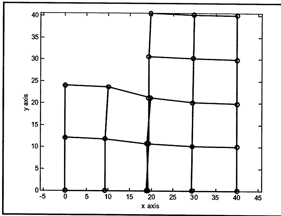
Figure 4.14. Deformed mesh after excavation with K_s = 1 \cdot 10^6 lb/ft (deformations magnified 10x)
