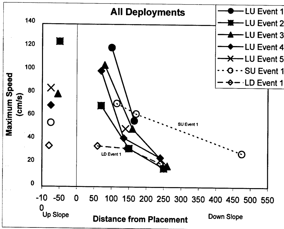
Figure 3-72. Observations of maximum surge current speed with distance away from cap load release point
