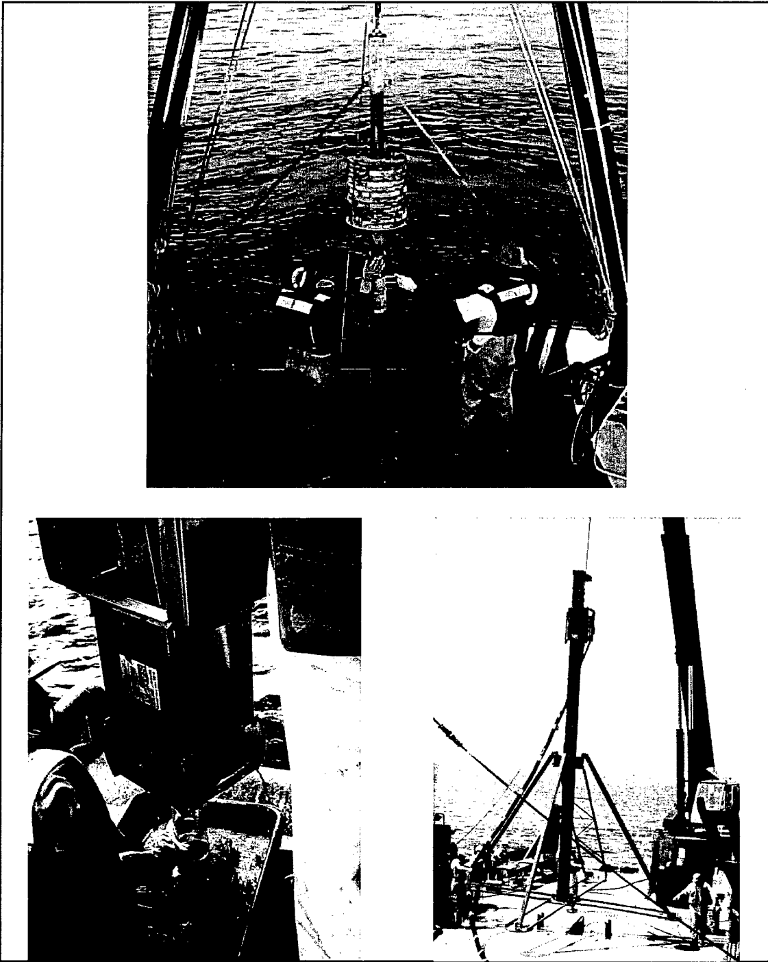
Figure 3-27. Types of coring equipment used for collecting sediment samples. Gravity corer (top), Gray-O'hara box corer (bottom left) and vibracorer (bottom right)
