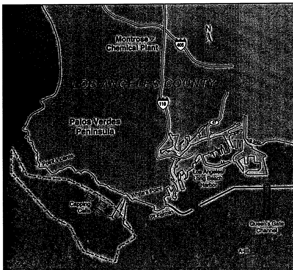
Figure 1-1. Location map showing Palos Verdes Shelf and slope, showing EA sediment footprint, pilot capping cells, Queen's Gate entrance channel, and borrow site A-III
