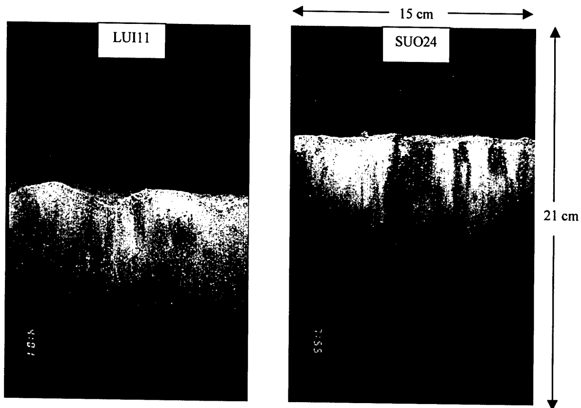
Figure 3-34. Comparison of representative SPI photos from landward (LUI11) and seaward cells (SUO24) showing difference in small scale topography resulting from biological burrowing activity
