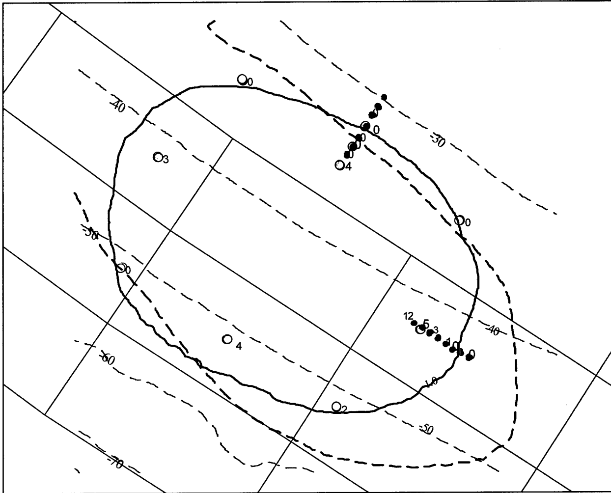
Figure 4-11. MDFATE LU71 hindcast simulation predicting maximum cap extent compared to SPI measurements. Solid black line is 1-cm contour from the MDFATE LU71 hindcast simulation without tidal currents, dashed black line is 1-cm contour from LU71 hindcast simulation with tidal currents. Colored dots are SPI cap thickness measurements, number next to dots are SPI cap thickness measurements
