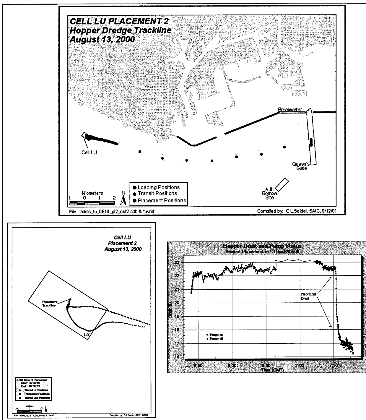
Figure 3-16. Example of dredge tracking information collected by Automated Disposal Surveillance System (ADISS). Top graphic shows the loading, transit, and placement positions. Left graphic shows detailed position during placement and right graphic shows time series of hopper draft during sequence
