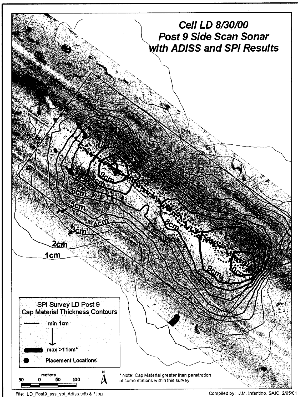
Figure 3-69. Side-scan sonar mosaic with SPI cap contours and ADISS dredge track – LD post 9
