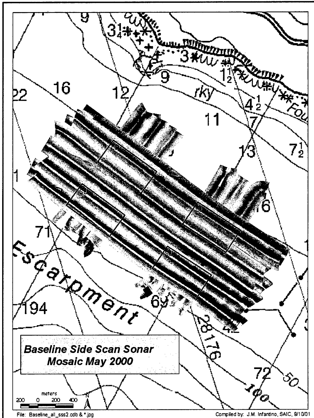
Figure 3-37. Baseline side-scan sonar mosaic showing relatively smooth, featureless seafloor
