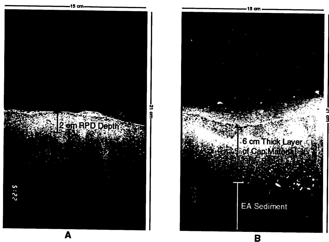
Figure 3-44. Two sediment-profile images from sta 108 to illustrate appearance of cap material layer on seafloor following single hopper placement event in Cell LU. Image A from background survey shows existing fine-grained sediment prior to cap material placement, with RPD depth of 2.0 cm. Image B from Post-1 survey shows distinct depositional layer of gray-colored, fine sand overlying existing fine-grained sediment at depth. Point of contact between cap material layer and underlying existing sediment is distinct. Light-colored, fine-grained sediment comprising the RPD in left image has been replaced, in effect, by depositional layer of capping sand at right
