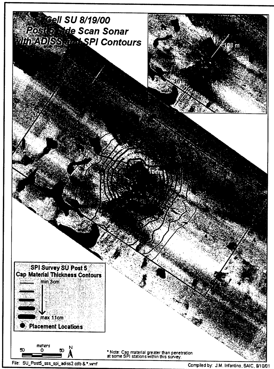
Figure 3-60. Side-scan sonar mosaic with SPI cap contours – SU Post 5. Inset shows central area of cell
