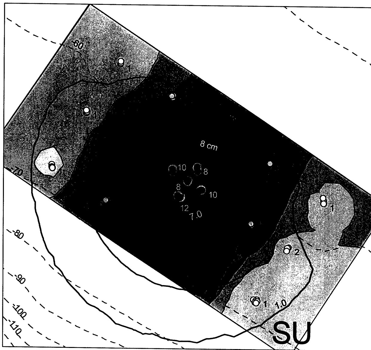
Figure 4-12. MDFATE hindcast simulation of SU5 and SPI inferred cap thickness (centimeters). MDFATE simulation had tidal currents and included stripping of sediments. Bold black lines are MDFATE cap thickness contours (x.0) in centimeters, colored dots indicate SPI stations, SPI cap thicknesses are in centimeters (whole numbers), pink dots behind colored dots are locations where cap thickness exceeded SPI penetration depth. SPI contours and color ramp (light to dark brown) are based on average thickness and are labeled as 2 cm, 4 cm, etc. Dashed green contours are water depths in meters
