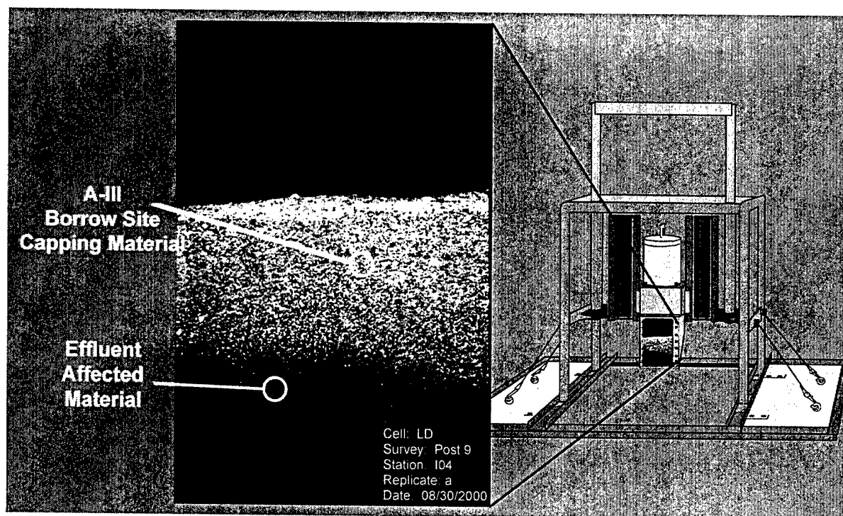
Figure 3-26. Schematic of sediment profile image (SPI) camera showing photo of profile down into sediment from Cell LD after placement of capping sand. Camera is able to photograph area 21 cm high by 15 cm wide. Plan view camera (PVC) was attached to frame of SPI camera so that it would take photograph before SPI touched seafloor
