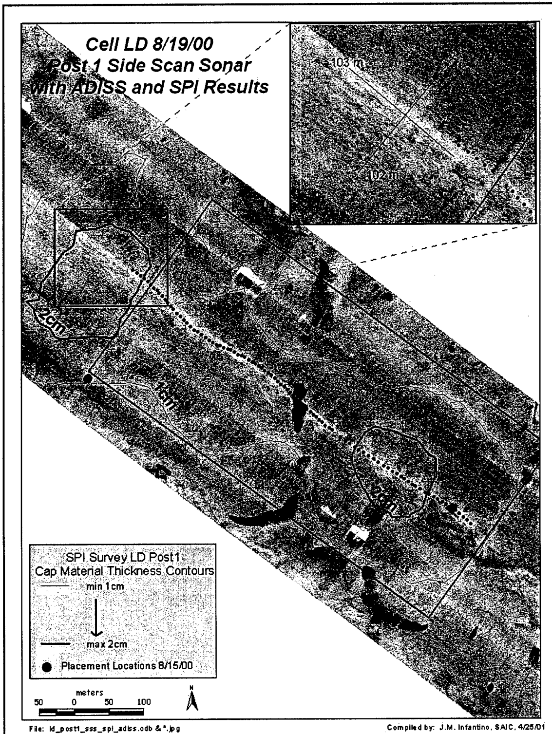
Figure 3-67. Side-scan sonar mosaic with SPI cap contours and ADISS dredge track – LD Post 1
