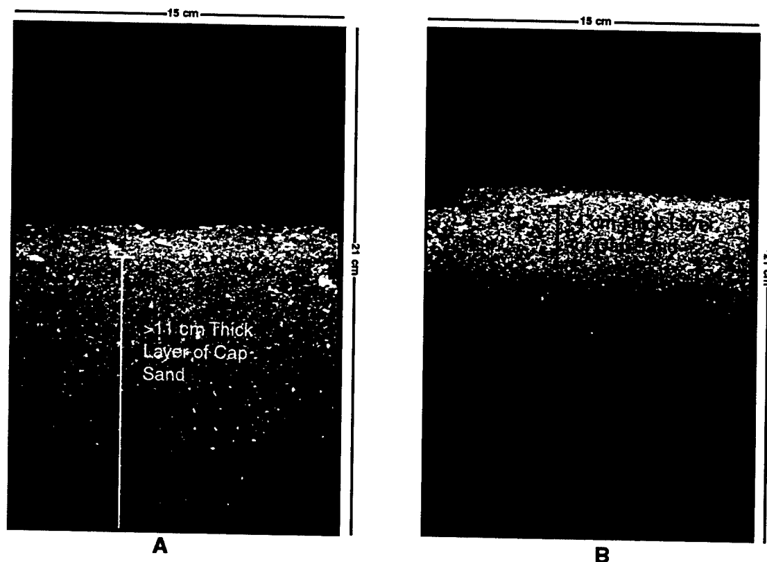
Figure 3-66. Representative sediment profile images from the Post-9 survey in Cell LD. Image A from a station along center line shows cap material from borrow site A-III (homogenous, golden sand) extending from sediment surface to below imaging depth (cap material thickness greater than penetration depth of 11 cm). Image B from station off center line shows discrete layer of golden cap sand measuring 4 cm thick
