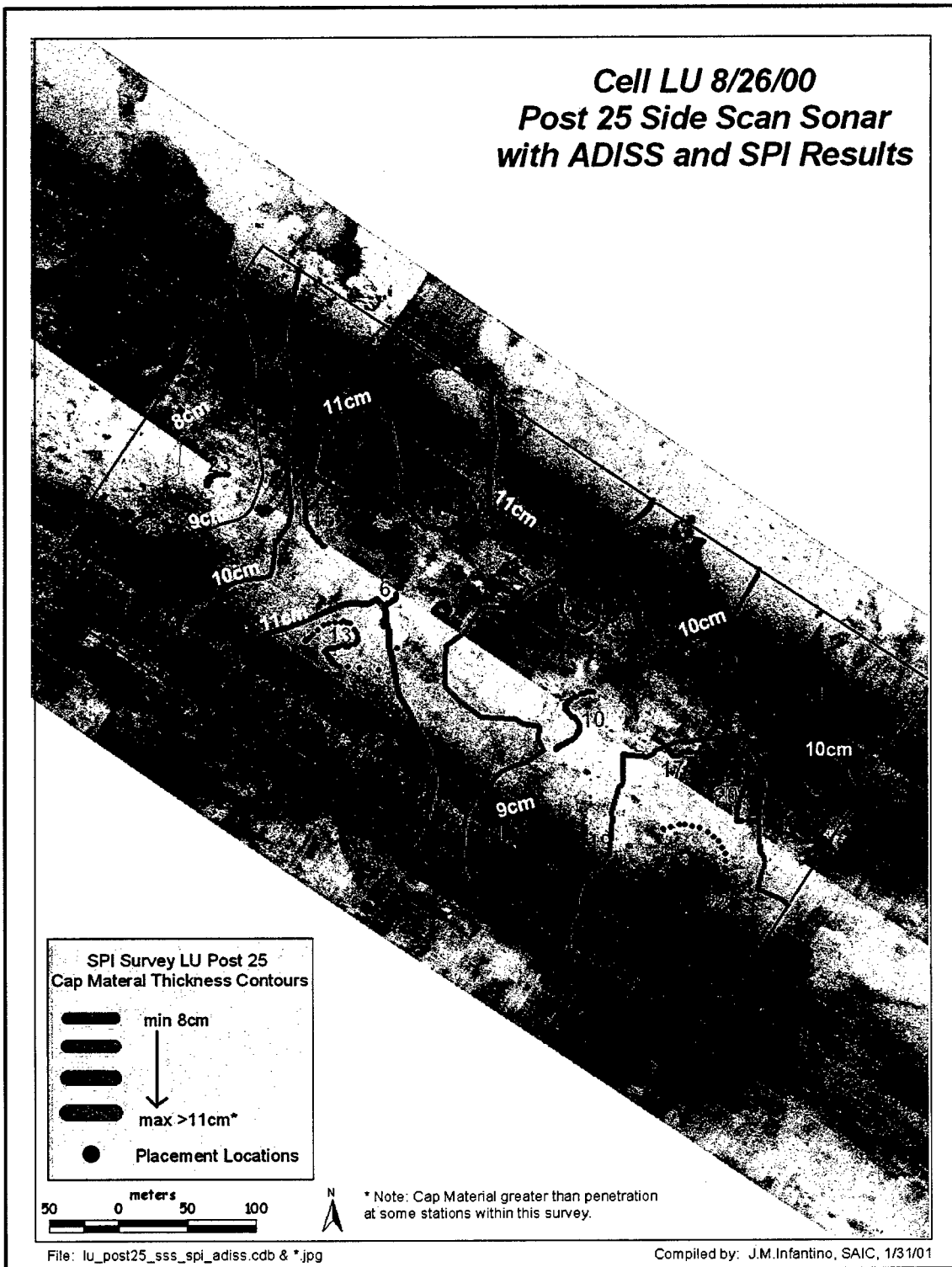
Figure 3-51. Side-scan sonar results after 25 placement events in Cell LU with SPI contours overlaid
