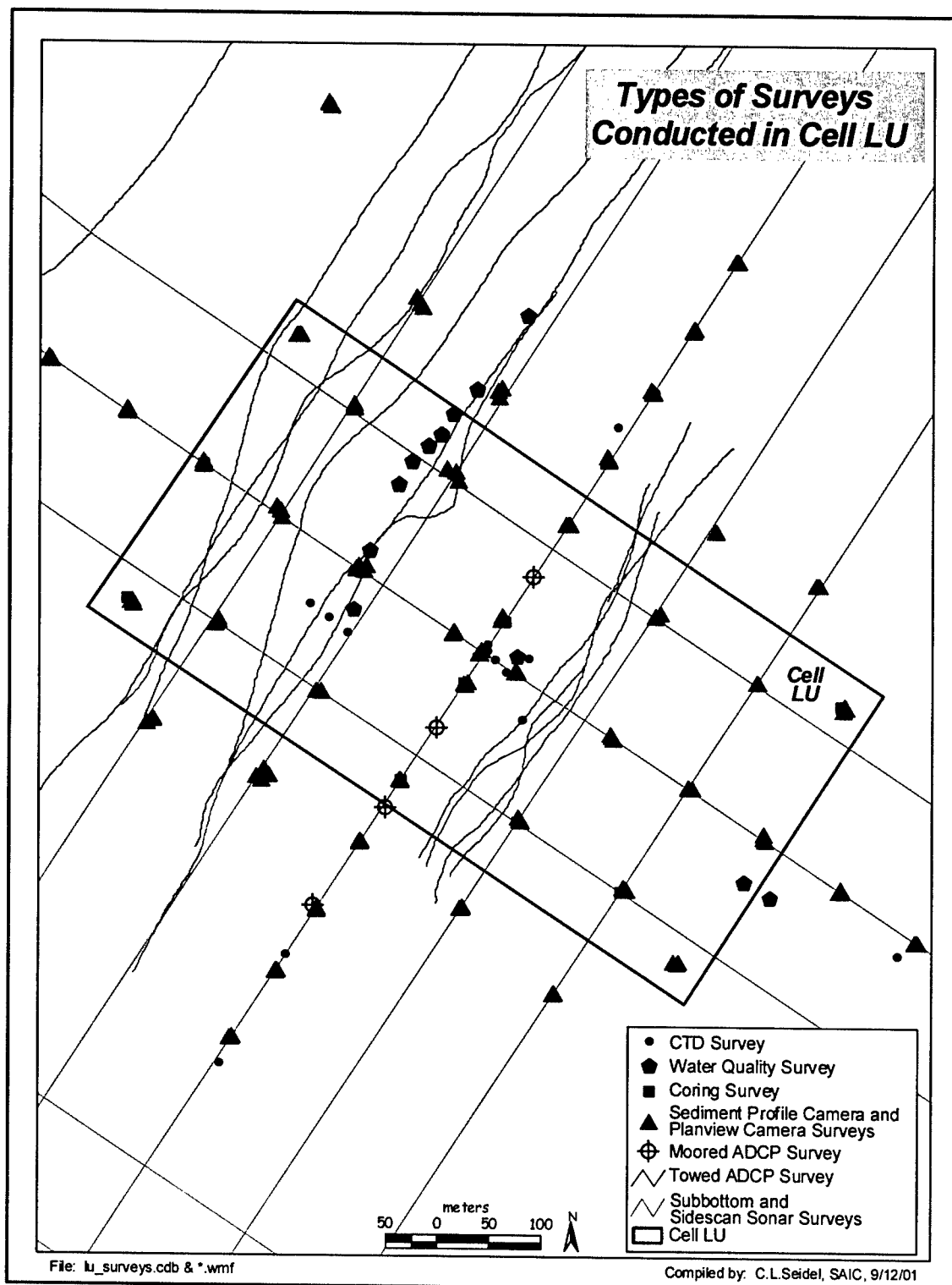
Figure 3-7. Composite graphic showing distribution of survey positions around Cell LU. Straight lines show the sub-bottom sediment profile and side-scan sonar tracks. Wavy lines show towed ADCP tracks during plume monitoring. Symbols indicate locations of bottom quadrapods, samples collected from the water column during plume tracking, and seafloor sample collection positions following cap placement events
