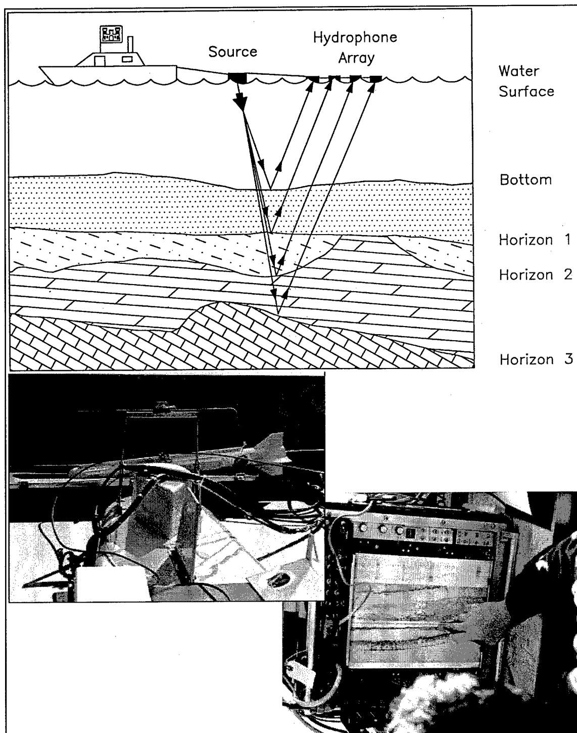
Figure. 3-25. Conceptual diagram of sub-bottom sediment profile operation along with photo (bottom left) of a sub-bottom fish in foreground (source) and example of sub-bottom recorder trace (bottom right)
