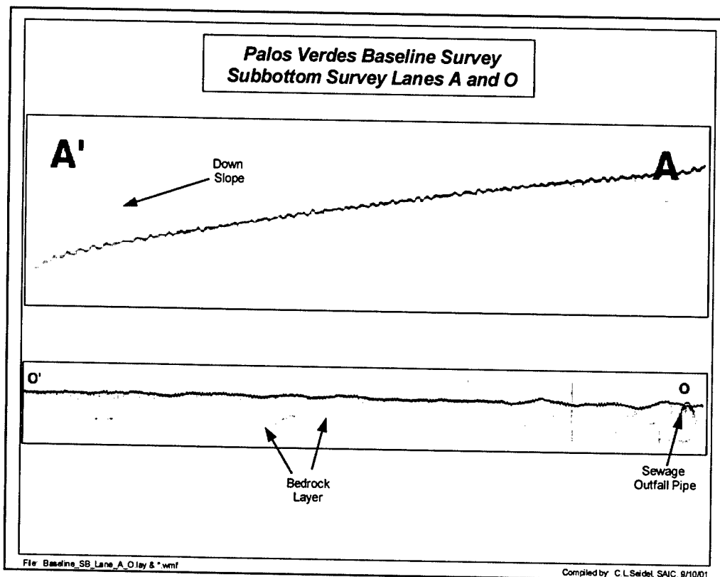
Figure 3-36. Examples of sub-bottom sediment profile survey data from baseline survey lanes A-A' and O-O'
