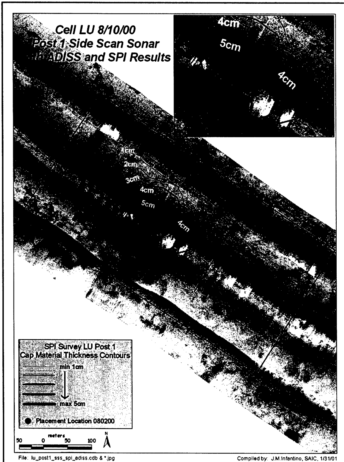
Figure 3-46. Side-scan sonar imagery after first load of cap material placed in Cell LU
