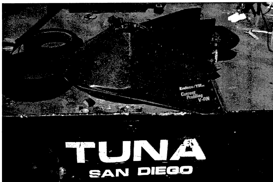
Figure 3-18. Acoustic Doppler Current Profiler (ADCP) towfish on deck of MV Tuna
