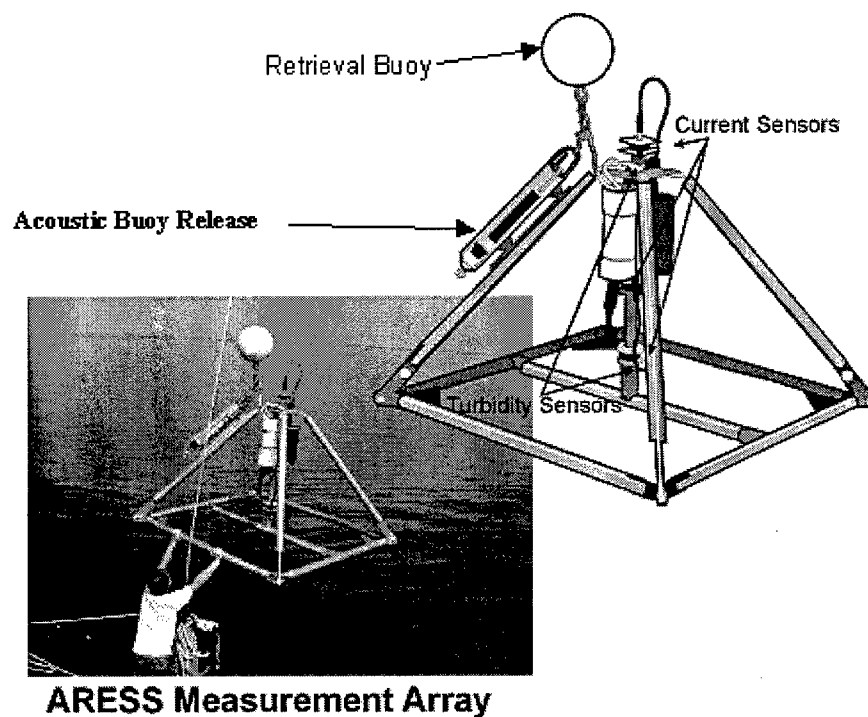
Figure 3-22. ARESS Oceanographic instrument array quadrapod
