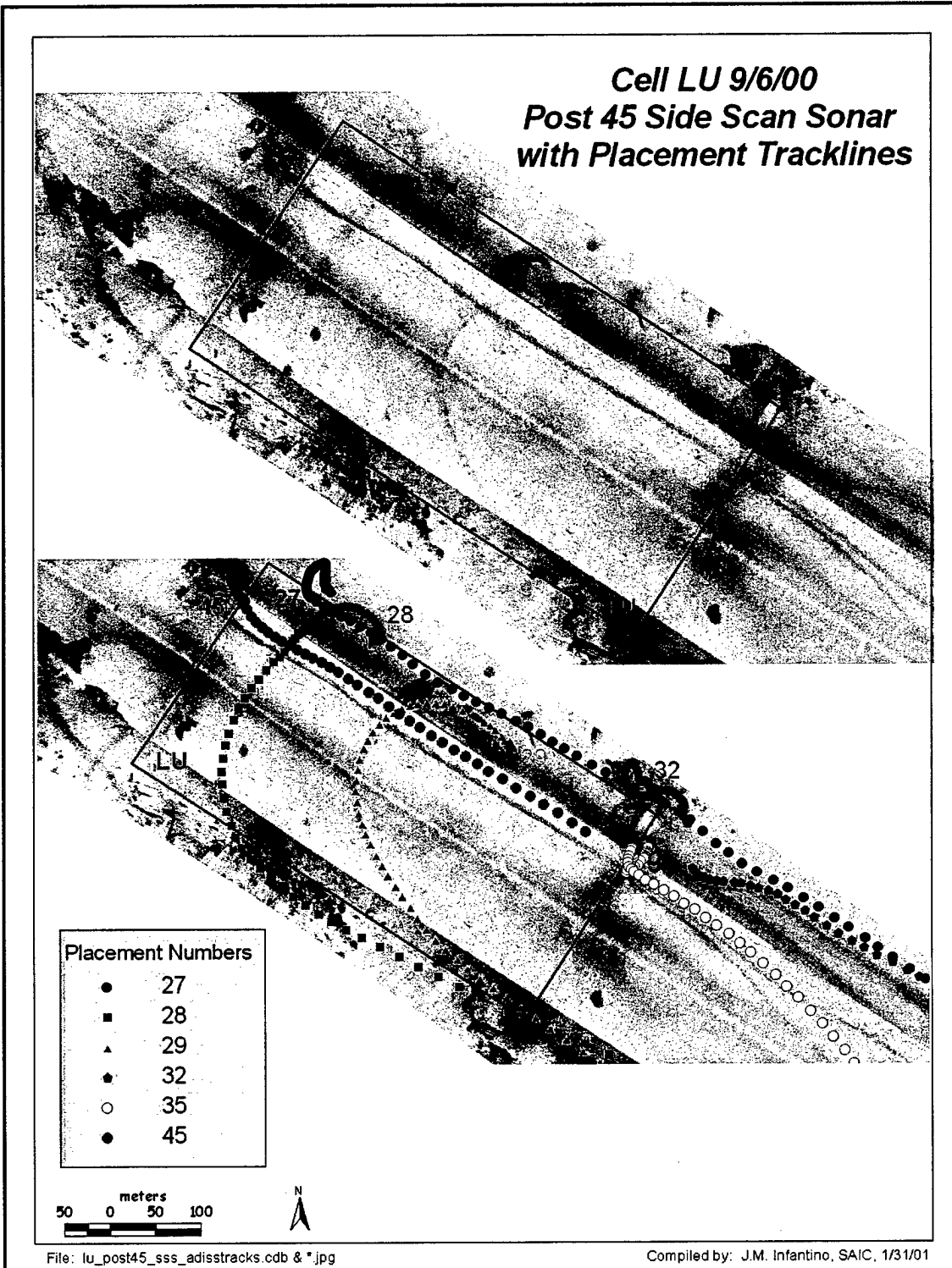
Figure 3-53. Side-scan sonar mosaic with dredge departure trails – LU Post 45
