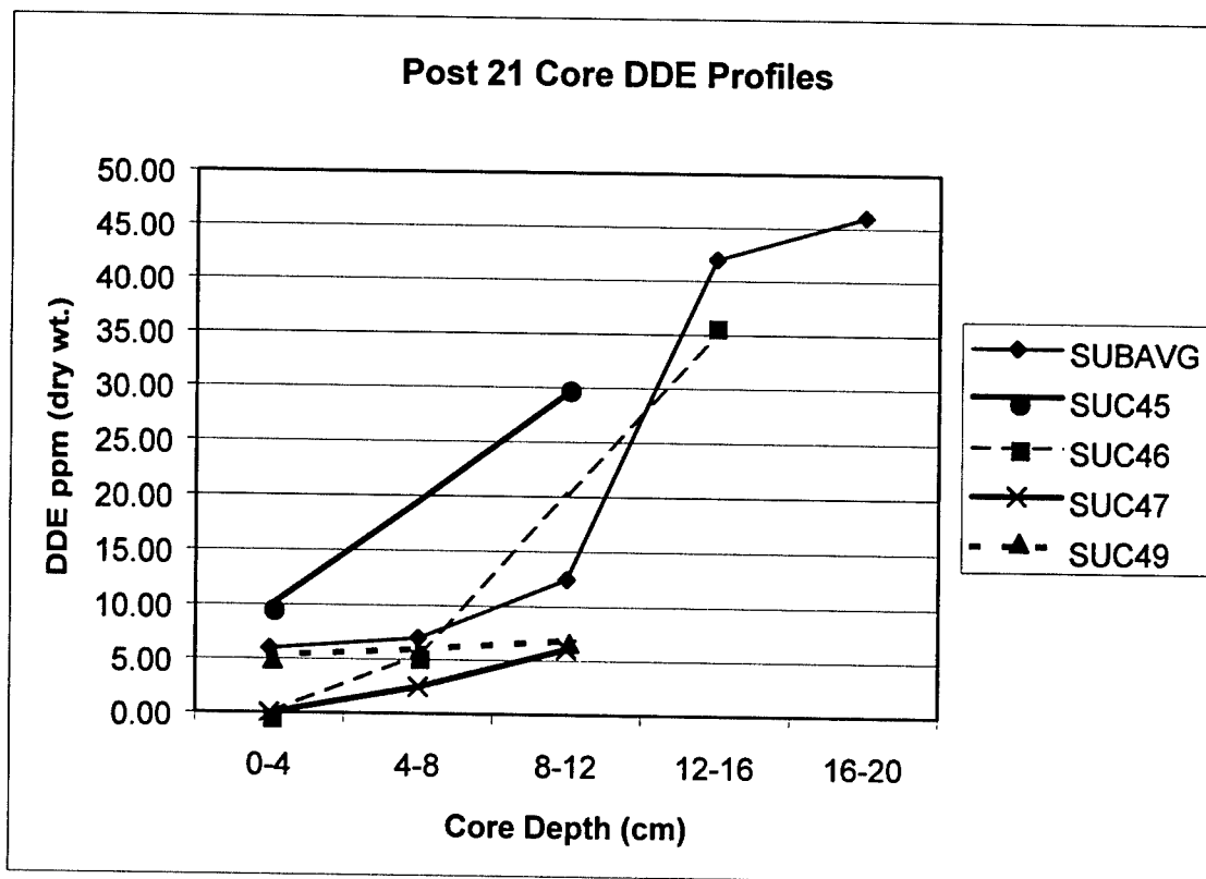
Figure 3-62. Down-core DDE concentrations in Post-21 cores in comparison to baseline (SUBAVG) EA sediment. Cores SUC46 and SUC47 were located on central portion of cap and cores SUC45 and SUC49 were farther out toward cap edge
