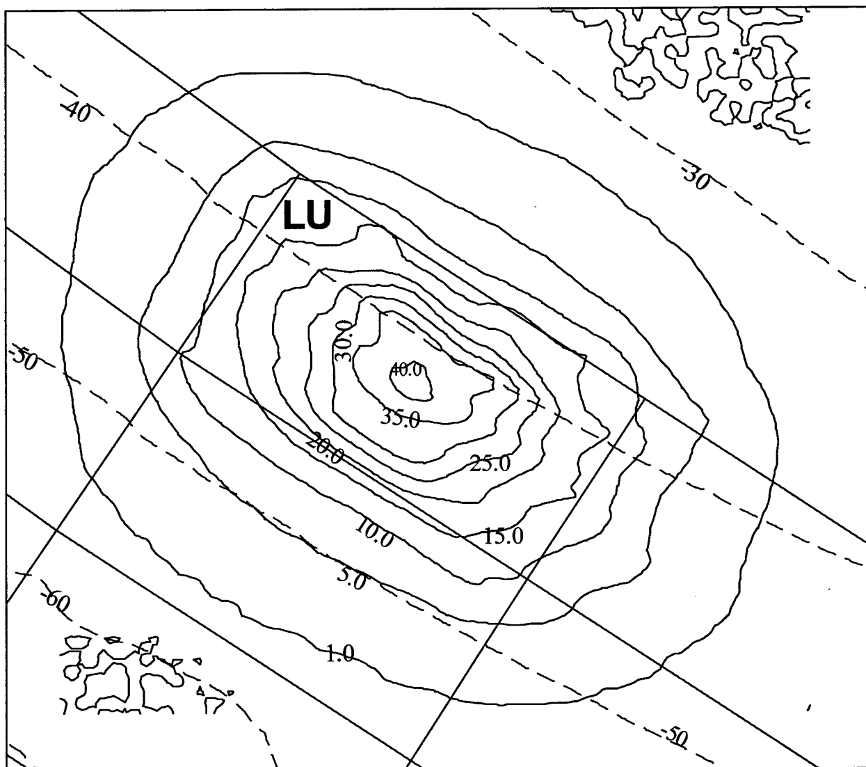
Figure 4-9. MDFATE simulation of LU71, without tidal currents, and including stripping of sediments. Solid contours are MDFATE cap thicknesses in centimeters, dashed contours are water depths in meters
