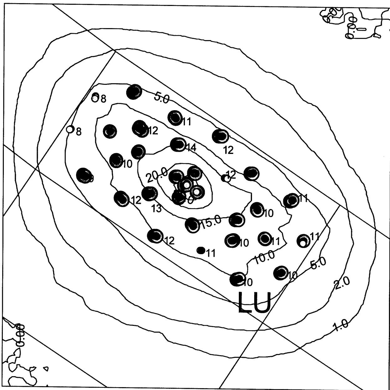
Figure 4-6. MDFATE hindcast simulation of LU25 and SPI inferred cap thickness (centimeters). MDFATE simulation had no tidal currents and included stripping of sediments. Solid lines are MDFATE cap thickness contours (x.0) in centimeters, colored dots indicate SPI stations, SPI thicknesses are in centimeters (whole numbers), pink dots are locations where cap thickness exceeded SPI penetration depth
