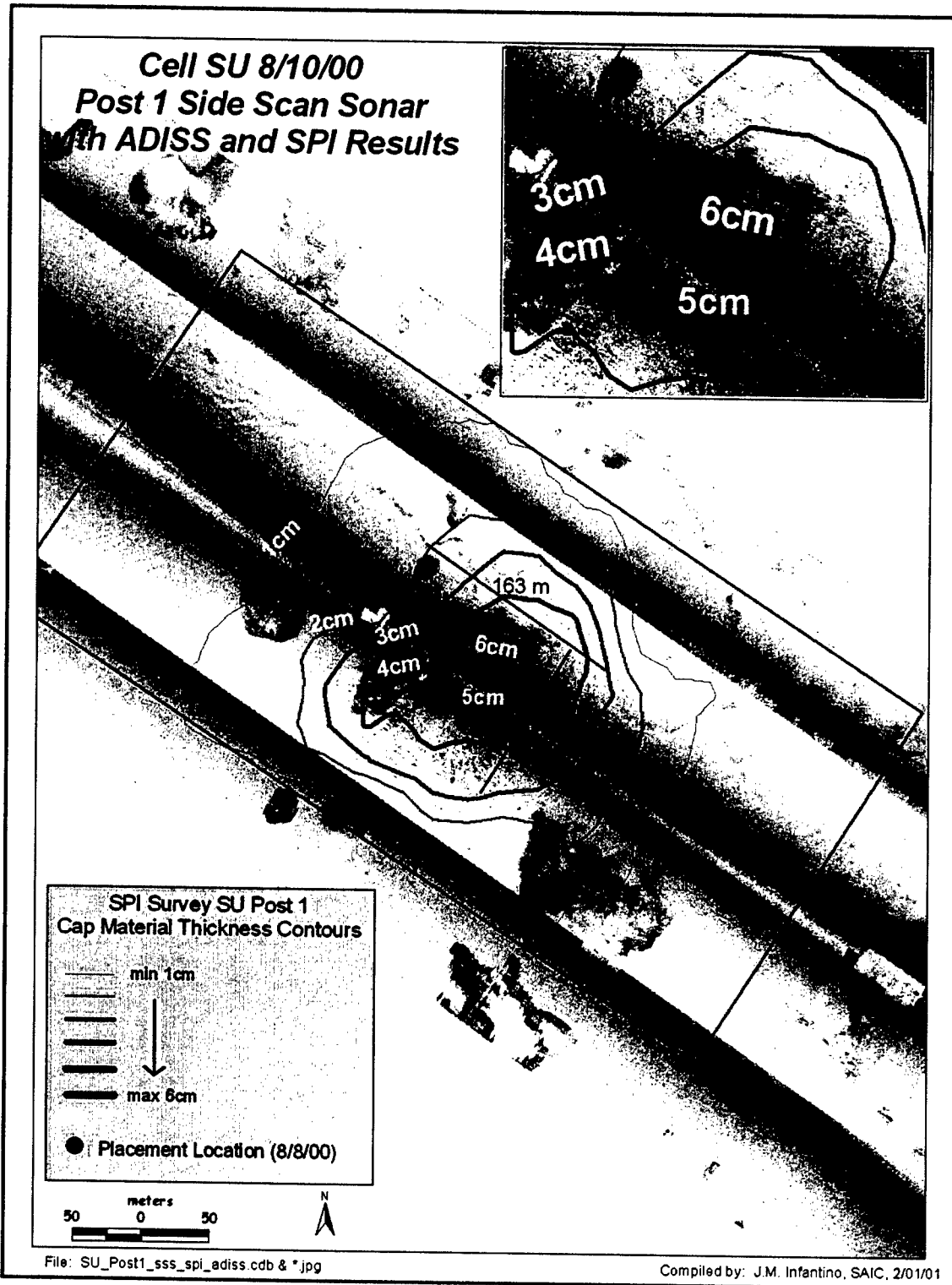
Figure 3-58. Side-scan sonar mosaic with SPI cap contours – SU Post 1
