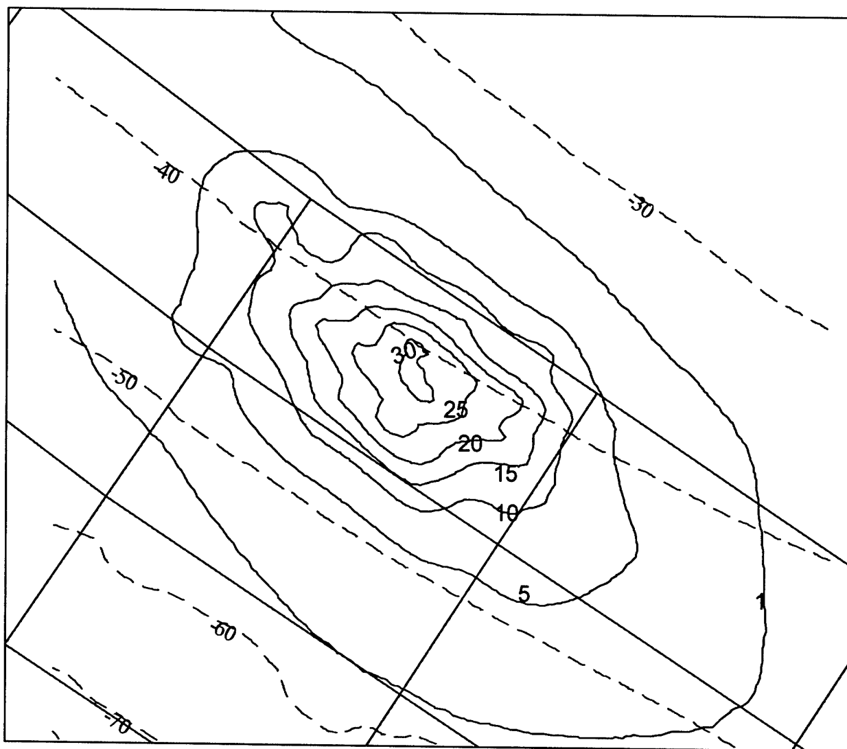
Figure 4-10. MDFATE simulation of LU71, with tidal currents, and including stripping of sediments. Solid contours are MDFATE cap thicknesses in centimeters. Dashed contours are water depth in meters
