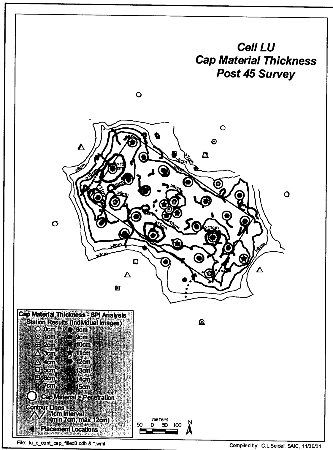
Figure 3-52. Distribution of cap determined by SPI camera after 45 placement events in Cell LU
