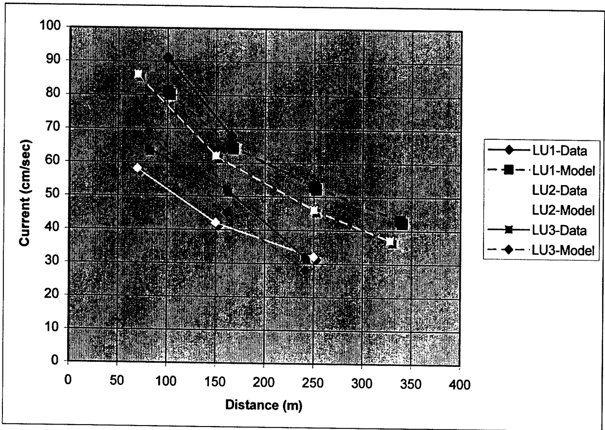
Figure 4-18. STFATE predictions (model) vs. measured bottom surge speeds (data) for placements LU1, LU2, and LU3
