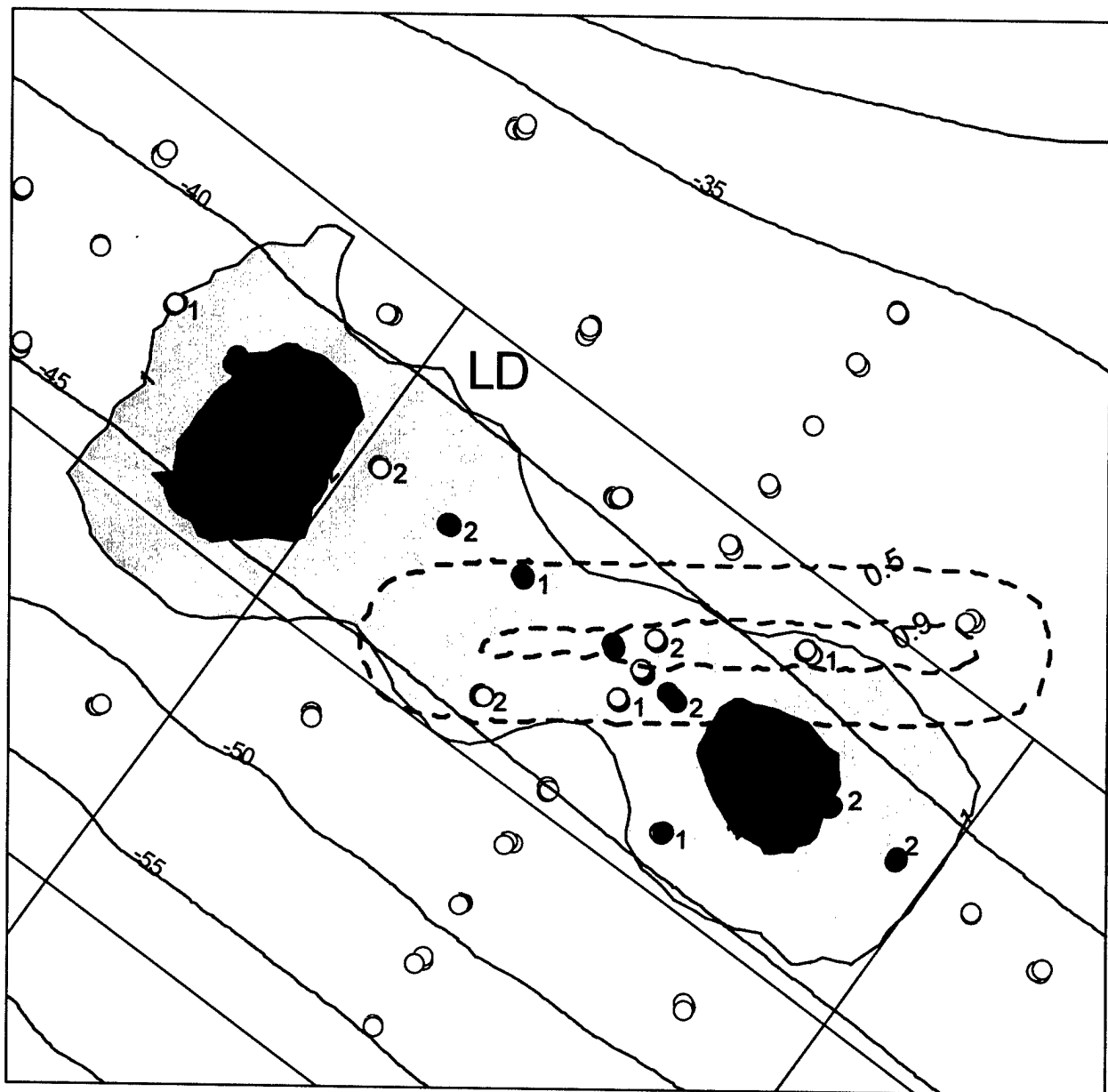
Figure 4-14. MDFATE hindcast simulation in spreading mode of LD1 placement and SPI inferred cap thickness (centimeters). Bold dashed lines are MDFATE cap thickness contours (x.0) in centimeters, brown dots indicate SPI stations, SPI thicknesses are in centimeters (whole numbers). SPI cap thickness measurements in centimeters are also indicated by brown color ramp and black contours, and labeled as integers. Water depth contours are in meters (e.g., -45)
