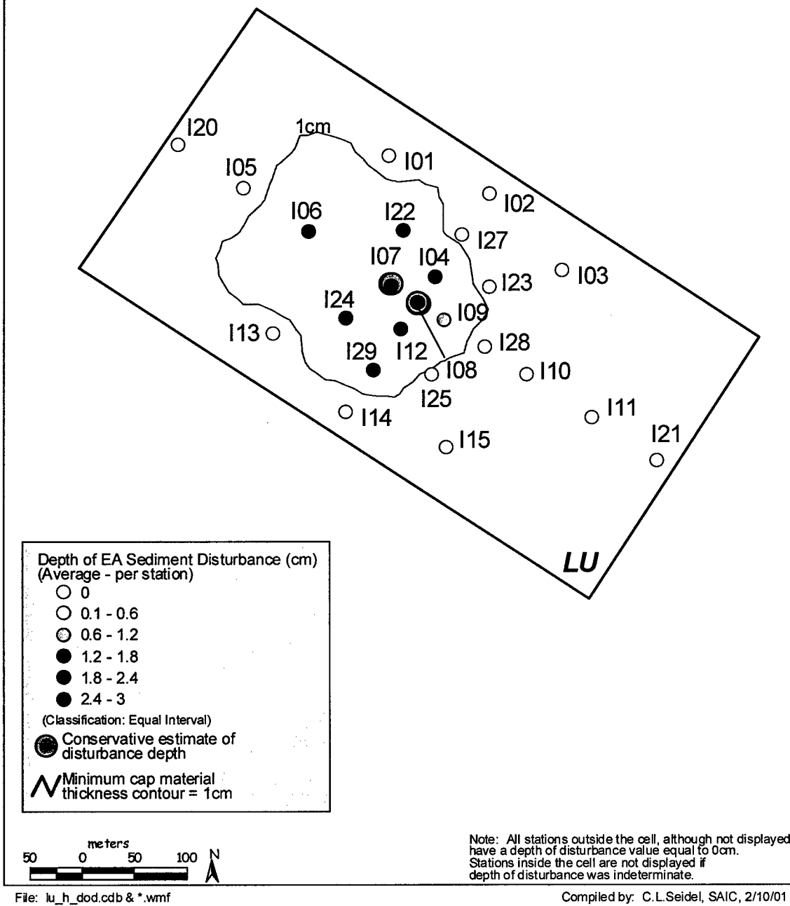
Figure 4-3. LU1 placement EA layer depth of disturbance based on SPI measurements (SAIC monitoring report)
