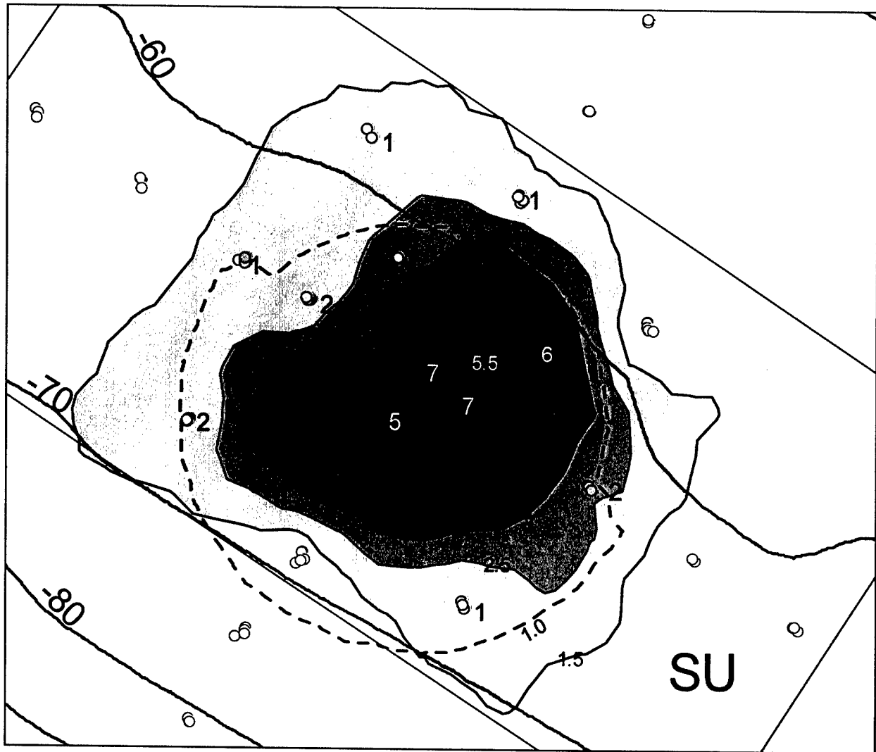
Figure 4-2. MDFATE hindcast simulation and SPI inferred cap thickness (centimeters) of initial SU placement. Dashed lines are MDFATE cap thickness contours (labeled with decimal, e.g., 1.0), solid lines are SPI cap thickness contours (labeled as decimal), colored dots show SPI station locations, labels next to colored dots are SPI cap thickness (integer), depth contours are in meters
