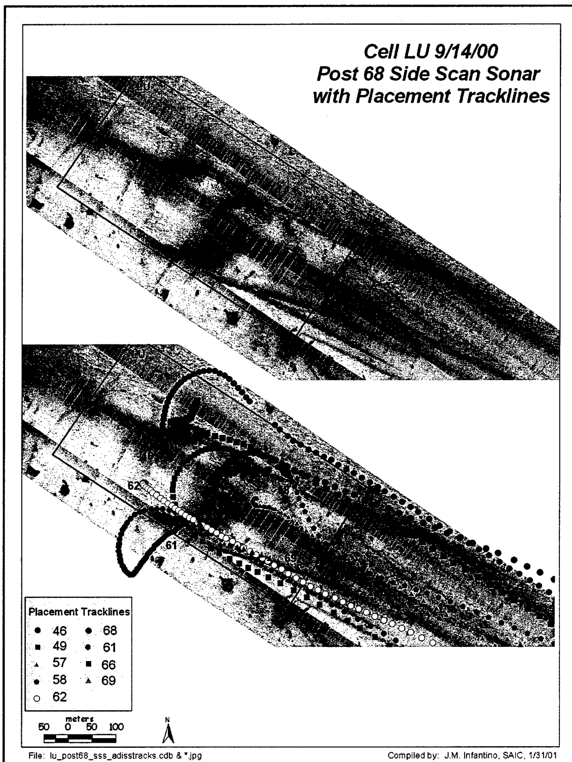
Figure 3-55. Side-scan sonar mosaic with dredge departure trails – LU Post 68
