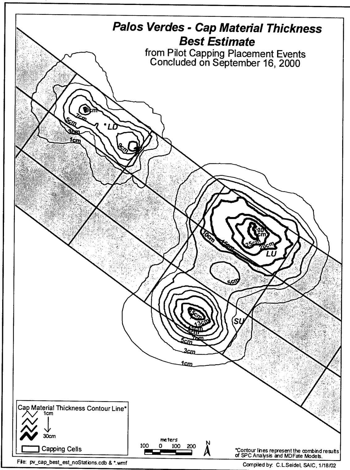
Figure 5-1. Estimate of total cap thickness as placed for the Palos Verdes pilot capping study
