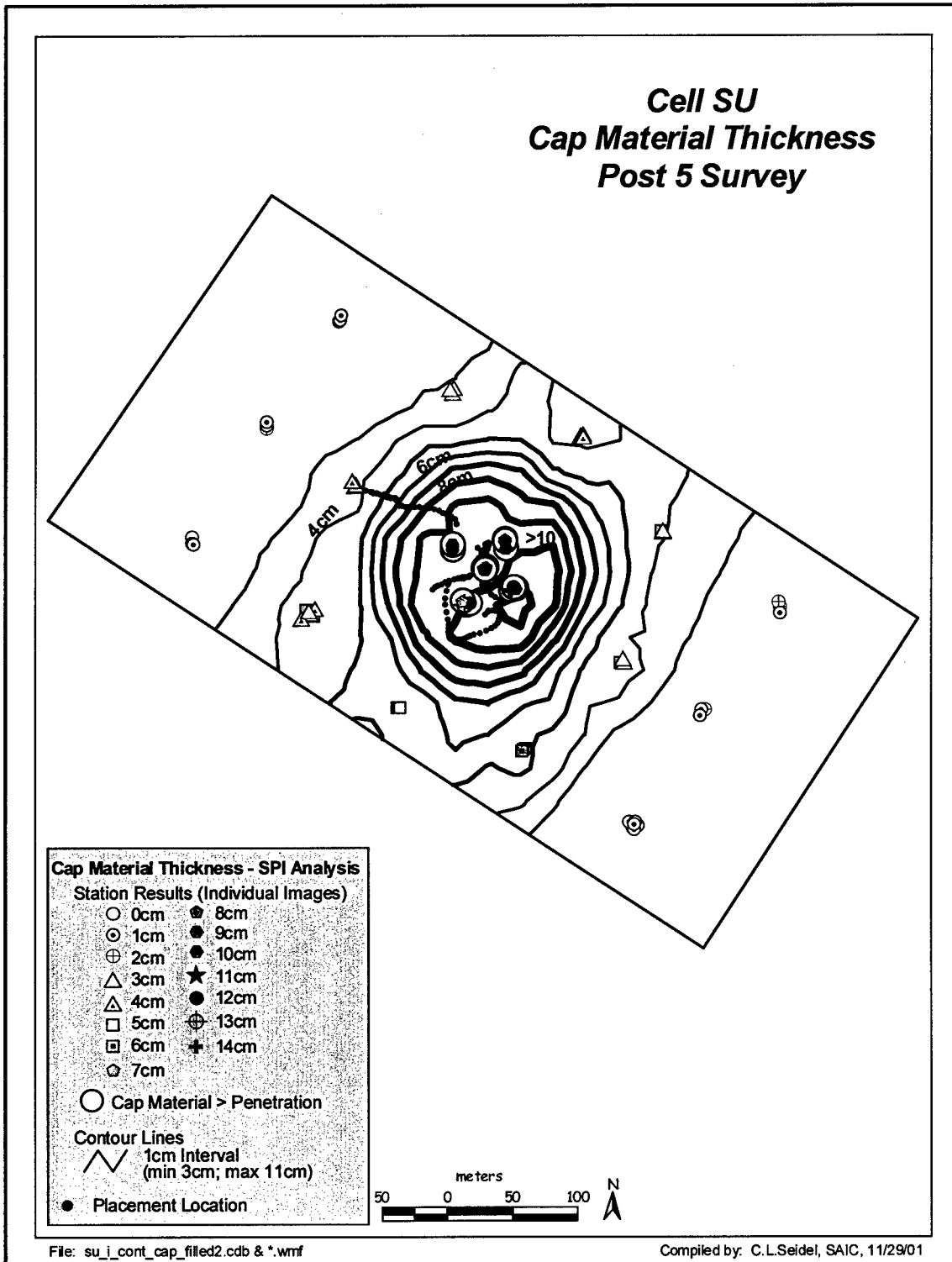
Figure 3-59. Placement locations and thickness of cap material on seafloor in Cell SU for Post 5 SPC survey. Contour lines are based on average measured thickness of cap material layer at each station (mean of n = 3 replicate sediment profile images), while each plotted symbol depicts cap material thickness measurement for individual replicate image. Note that cap material layer thickness exceeded penetration depth of sediment profile camera in a number of images near center of the cell (cap material > penetration)
