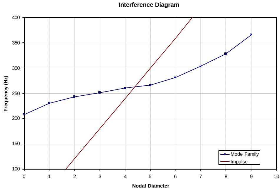
Figure 7 Interference diagram showing 4 disk effect modes belonging to one family
