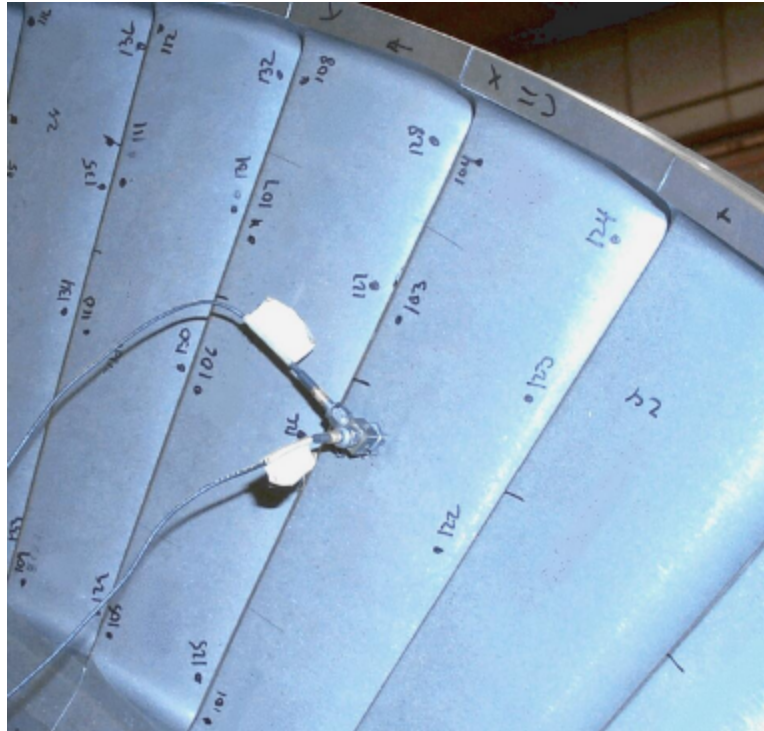
Figure 5 Accelerometer Configuration
