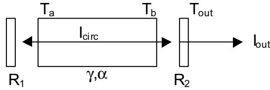
Figure 2-3 Standing Wave Laser Cavity For Laser Model
