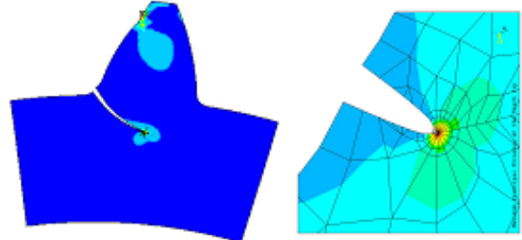
Figure 6 – 2-D Finite Element Model
