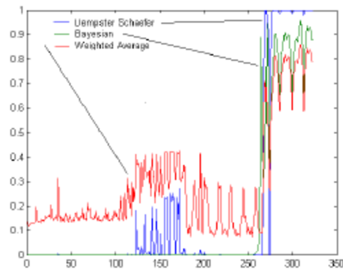
Figure 14 - Feature Fusion
