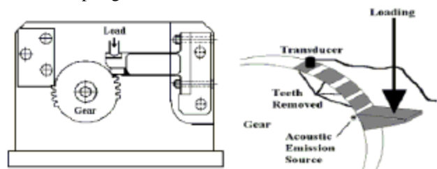
Figure 2 – Single Tooth Test Rig
