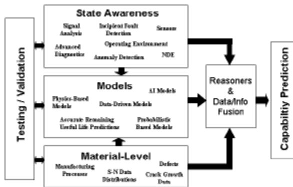
Figure 1 – Capability Prediction
