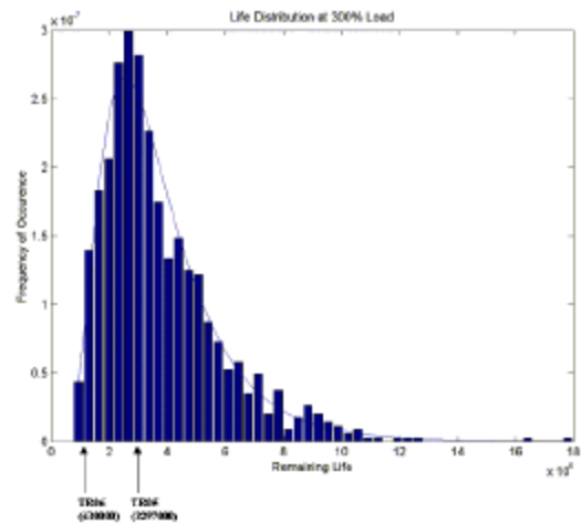
Figure 12 – Validation on 2 runs at 300% load
