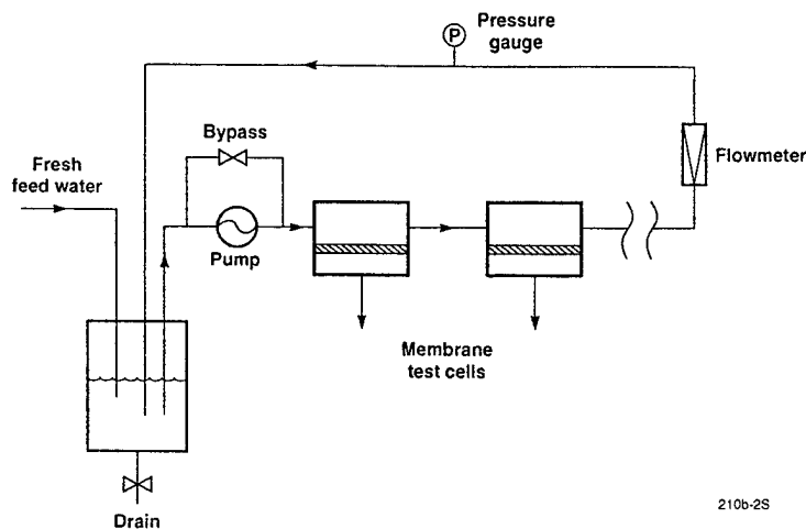
Figure 9. Simplified flow schematic of cross-flow test system with multiple test cells in series.
