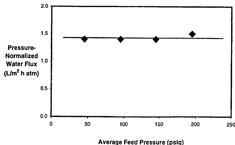
Figure 16. Pressure-normalized water flux of a Pebax 1074 module (#1510) as a function of average feed pressure. Feed solution: pure water; feed temperature: 21 °C; feed pressures: 50, 100, 150 and 200 psig. Feed spacer: Nylon ROF030; permeate spacer: double Tricot 9944.
