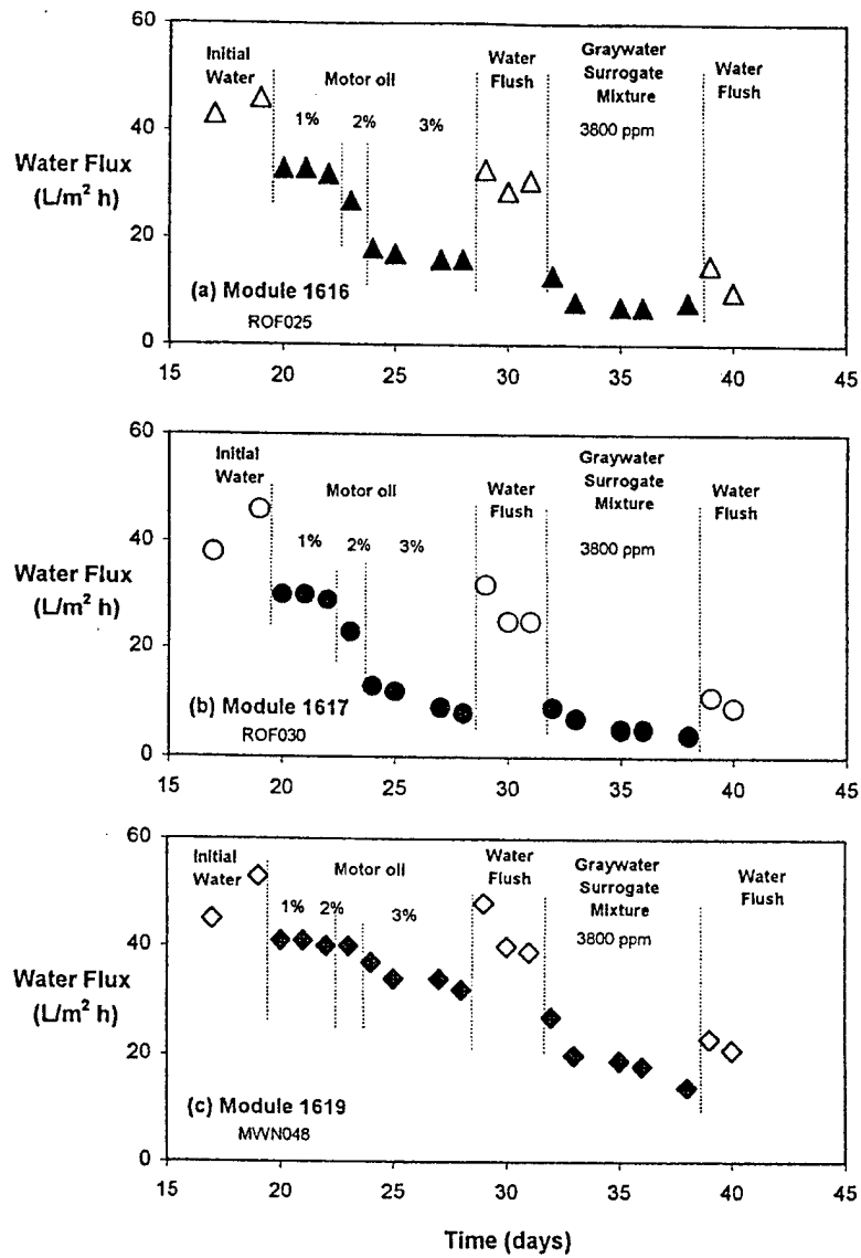
Figure 19. Water fluxes as a function of operating time for Pebax 1074/PVDF modules: (a) 1616 with an ROF025 spacer, (b) 1617 with an ROF030 spacer, and (c) 1619 with an MWN048 spacer. Temperature: 23 °C; pressure: 150 psig; feed-to-residue pressure drop across module: 10 psig.
