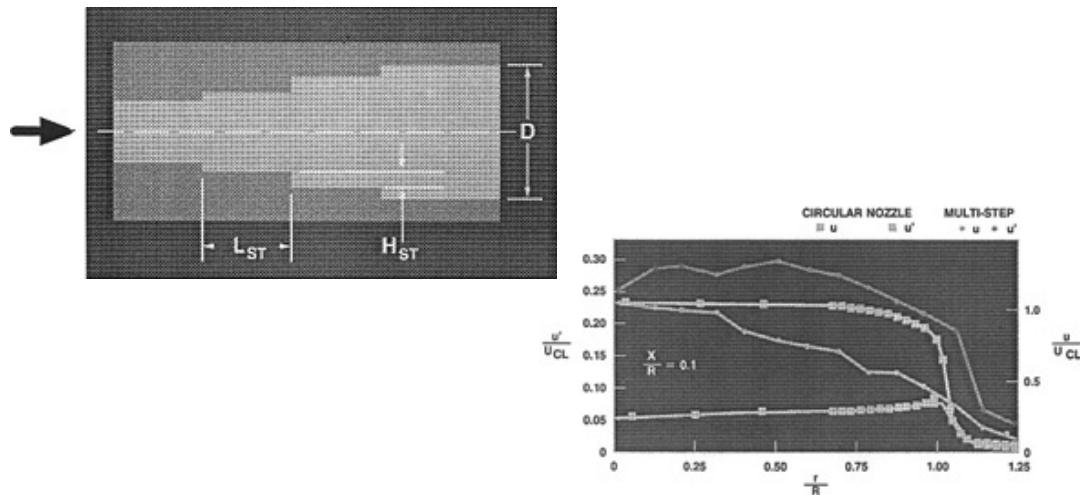
Figure 17. Fine-Scale Turbulence Enhancement in Multi-Step Nozzle.
