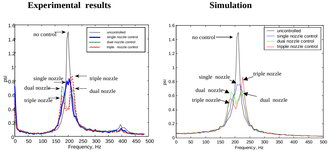
Figure 20: PSD of pressure signal with on-off control of one, two, or three liquid fuel nozzles. The peak splitting phenomenon observed in experiment and simulation.
