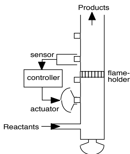
Figure 2. Typical active control demonstration experiments using a simple tube combustor.
