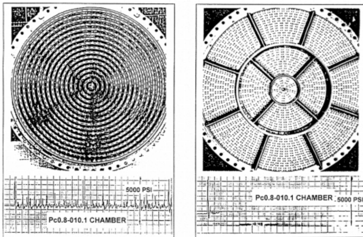
FIGURE 8.1. Examples of Baffles in the F-1 Liquid Rocket Engine
