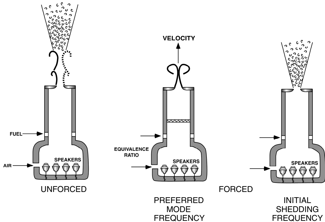
Figure 27. Forced Premixed Flame for Extension of Flammability Limits.
