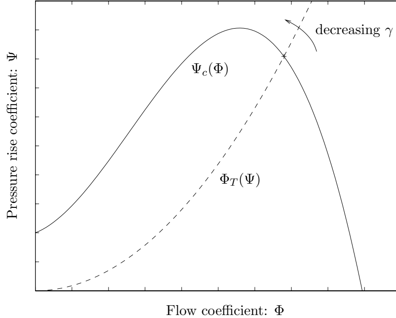
Figure 6: Compressor and throttle characteristic curves.
