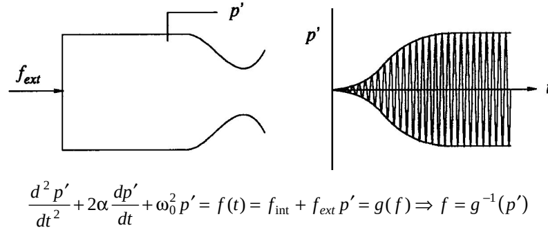
Fig. 2 Pressure oscillations in a combustion chamber.
