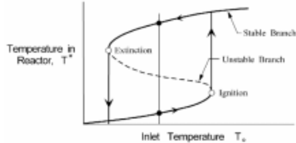
FIGURE 7.10. Hysteresis Loop for a Recirculated Zone Idealized as a Simple Chemical Reactor
