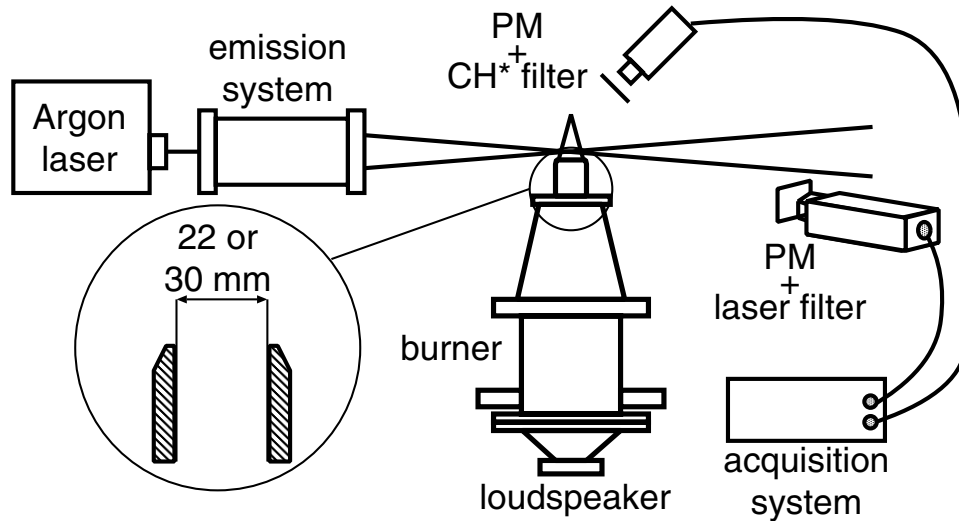
Figure IV.2: Experimental Setup.
