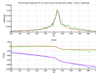
Figure 18: Frequency responses of pressure to valve command in UTRC sector rig experiment.
