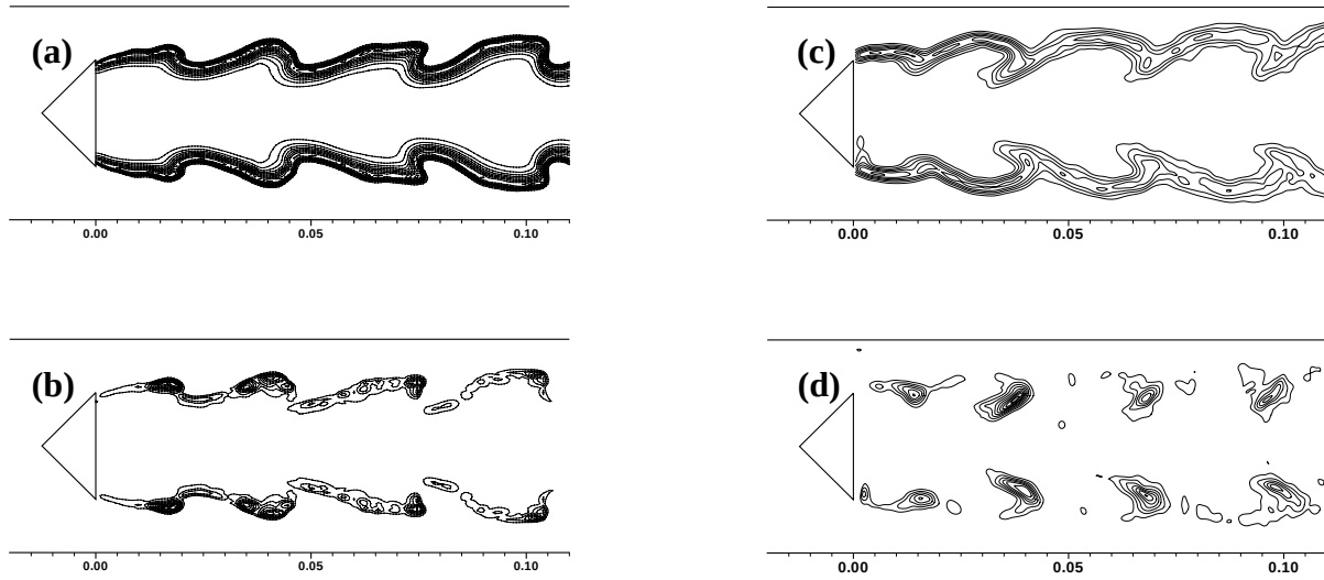
Figure IV.9: Acoustically excited ( f_e = 870 \text{ Hz} ) turbulent premixed flame at phase 2\pi/3 , relatively to the microphone pressure signal. Large eddy simulations fields of the instantaneous reaction rate. (a) total fuel reaction rate, E\dot{\omega}_F/F , in Eq. (IV.48). (b) modeled subgrid scale contribution, (E - 1)\dot{\omega}_F/F . Corresponding experimental data (20 images, corresponding to the same phase, have been averaged to ensure statistical stability of the unresolved contributions): (c) total fuel reaction rate, \rho_u s_l^0 Y_F^0 \Sigma = \rho_u s_l^0 Y_F^0 \Xi |\nabla \bar{c}| ; (d) unresolved subgrid scale contribution \rho_u s_l^0 Y_F^0 (\Xi - 1) |\nabla \bar{c}| .
