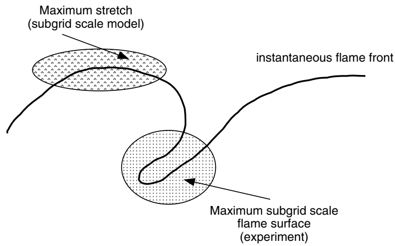
Figure IV.11: A rough scheme comparing regions of maximum values of the unresolved reaction rate in numerical prediction and in experimental data. Maximum contributions of the subgrid scale model are observed in the stretched regions because of the subgrid scale velocity fluctuation detection (Eq. IV.50). Experimental results display maximum values of the wrinkling factor \Xi at the vortice head where highly curved intantaneous flame fronts are not resolved on the filtered flame front.
