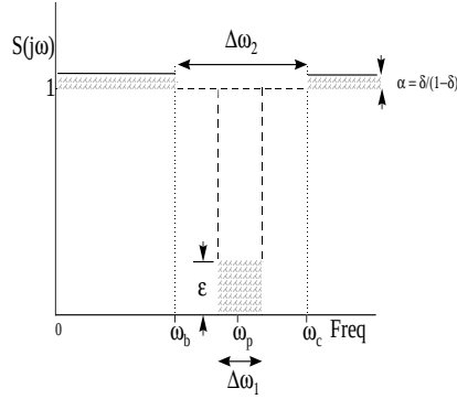
Figure 12: Performance specification for finite bandwidth control : |L(j\omega)| \leq \delta(\frac{\omega_c}{\omega})^{1+k} for frequencies \omega > \omega_c . \delta < \frac{1}{2} and k > 0 (relative degree of at least two) and |L(j\omega)| \leq \delta(\frac{\omega}{\omega_b})^{1+k} for frequencies \omega < \omega_b .
