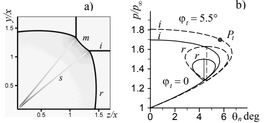
Fig. 4. Cross flow pattern of vNR-type (a) and shock wave polars (b) for M = 1.5 , \theta_w = 5^\circ , \nu = 90^\circ , \chi = 0 .
