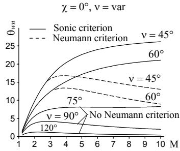
Fig. 10. Transition wedge angles for corner configurations with different dihedral angles.
