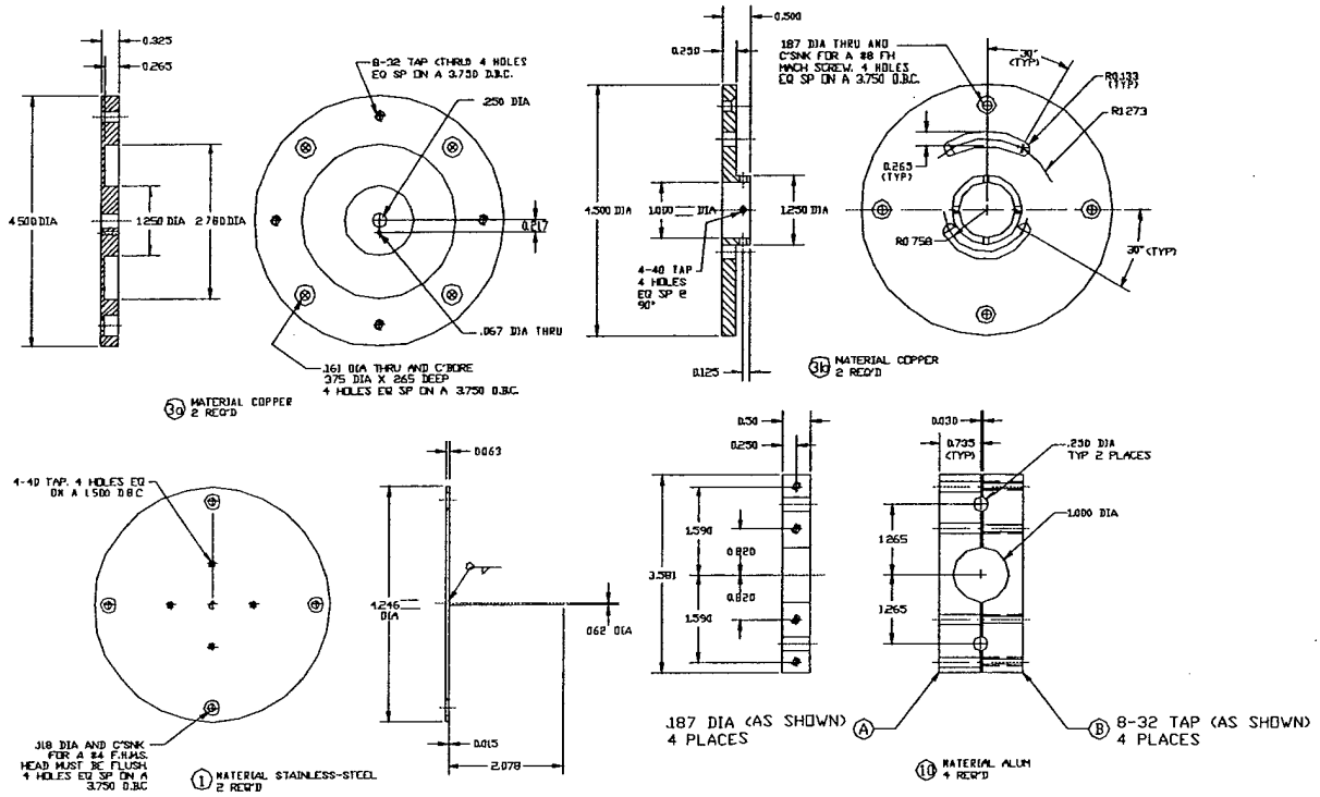
Figure 8 Metal pieces for head of etching stage assembly. All dimensions are in inches.
