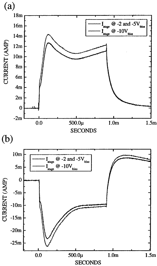
Graph 2 Temporal dependence of stage currents measured through (a) load resistor and (b) Pearson coil at various dc bias levels
