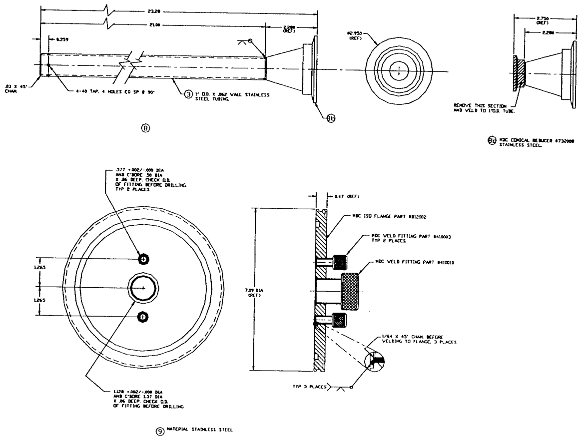
Figure 9 Shaft and mounting flange for etching stage. All dimensions are in inches.
