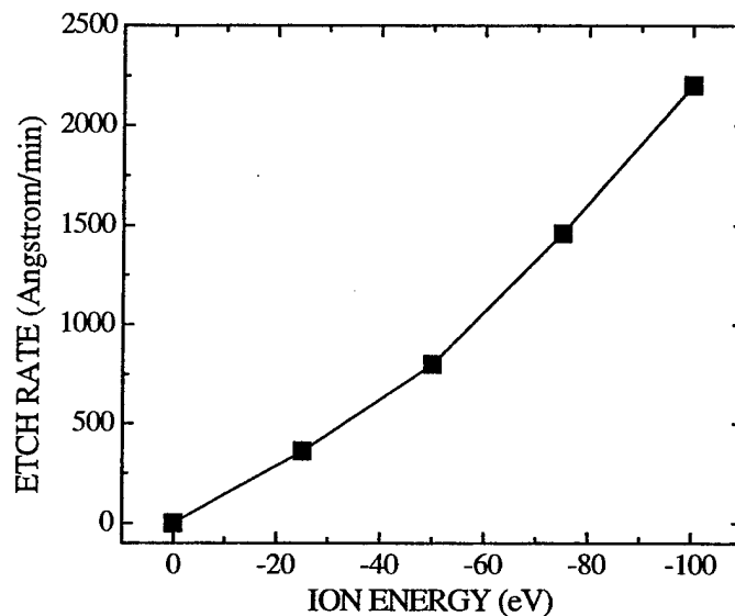
Graph 6 ER of negative resist material versus ion energy
