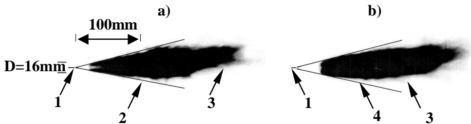
Fig. 5. Image of torch. a) – large exposition, b) – small exposition. 1 – nozzle, 2 – envelope of flame front, 3 – torch bound, 4 – bound of the jet boundary layer. Q = 2.3 l/s, injector diameter is of 1.2 mm.
