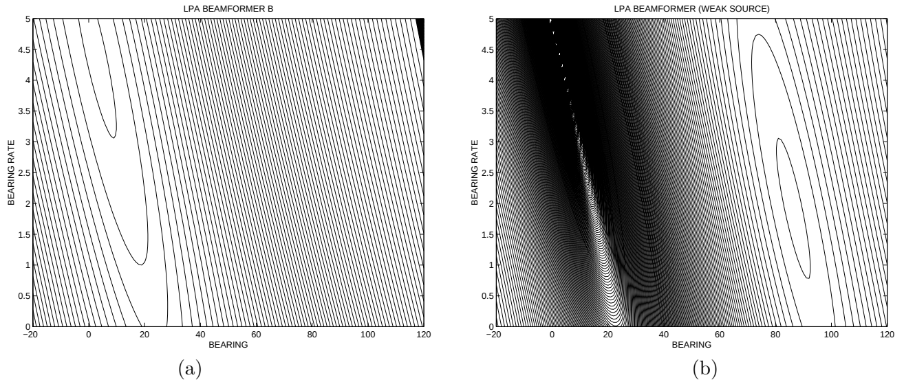
Figure 6: (a) Beam pattern of LPA beamformer, showing the location of the stronger source (M3). (b) Beam pattern of LPA beamformer after subtracting an estimate of the strong source signal from the data, showing the location of the weaker source (M1).
