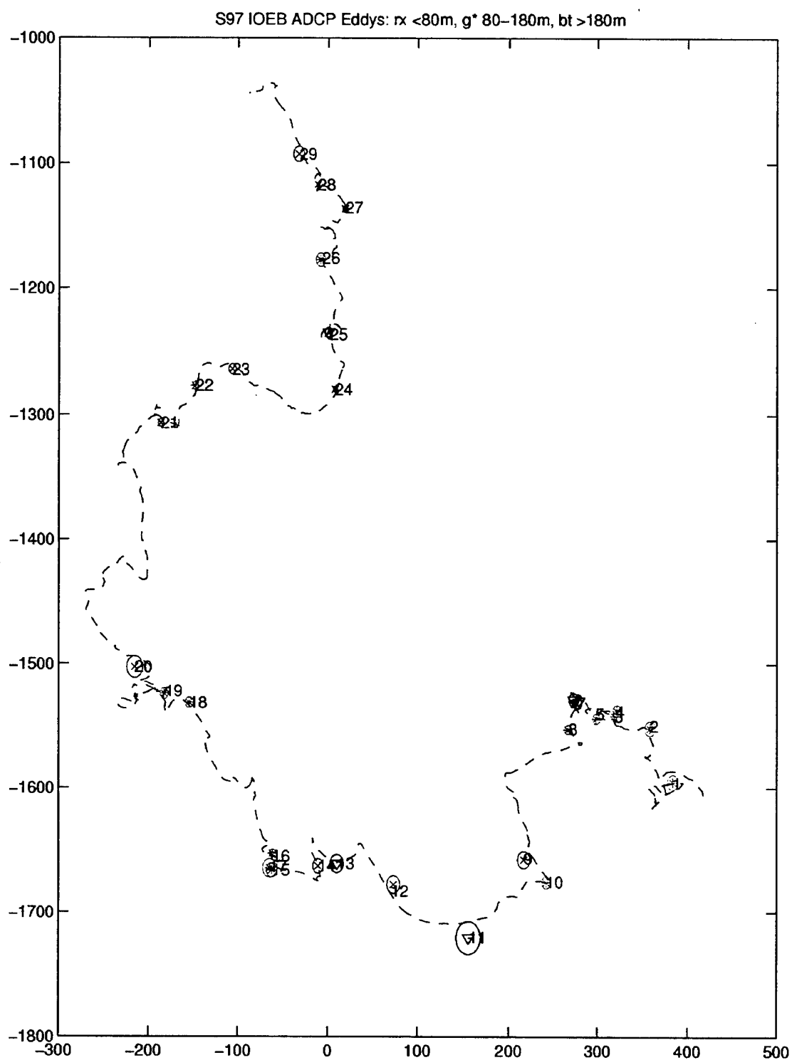
Figure 79. S97 eddies on IOEB drift track converted to a Cartesian coordinate system with diameters indicated by circles, and depths indicated by marks: shallow = x, halocline = *, deep = triangle.
