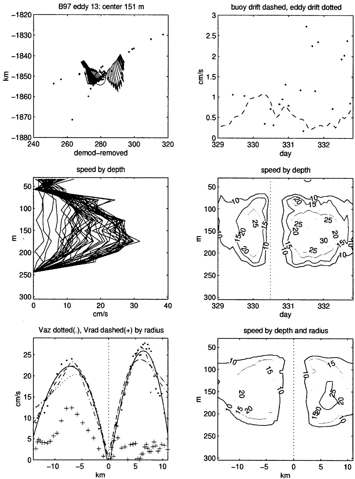
Figure 73. B97 eddy 13 plot of velocities in space, time, and by radius.
