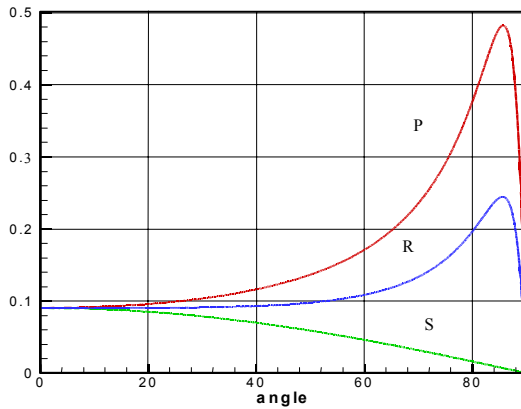
Fig. 3. Dependence of the radiation absorption factor on the incident angle at different polarization ( S - perpendicular, P - parallel, R - circle).
