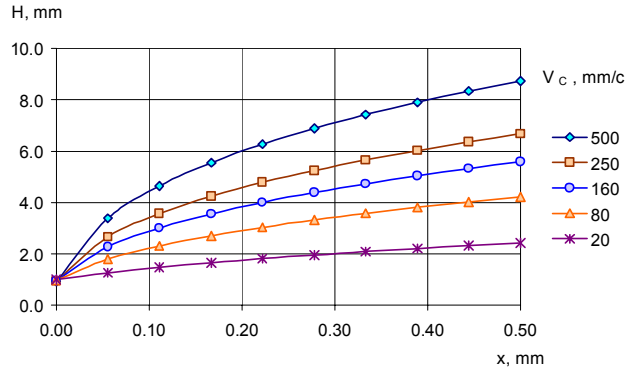
Fig. 2. Influence of the cutting velocity on thickness of the liquid melt layer.
