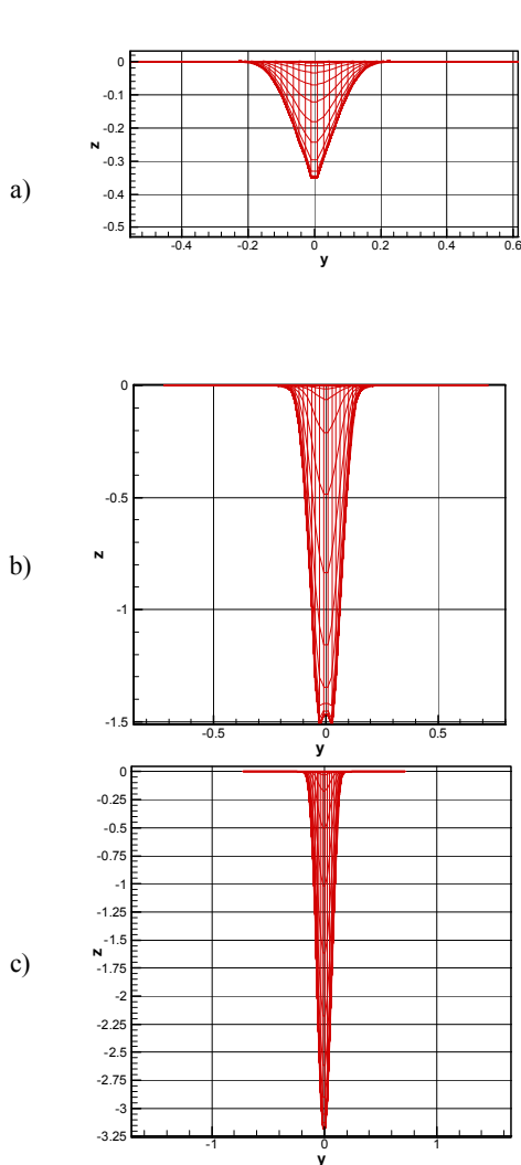
Fig. 4. Influence of the radiation polarization on the cutting depth and form: a) S – perpendicular; b) R –circle; c) P –parallel ( z_f = 0 ).
