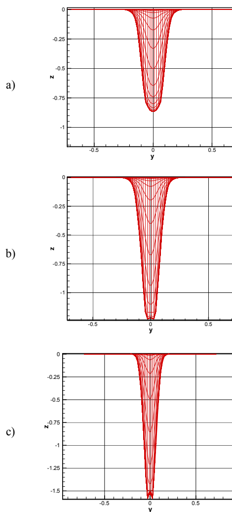
Fig. 5. Influence of the deepening of the focus on the cutting form (circle polarization): z_f mm: a) +3 mm; b) –1 mm; c) –3 mm.
