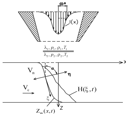
Fig. 1. Interaction of the gas jet and radiation with the metal plate.
