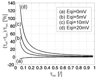
Fig. 5: Error in the overheating estimation
