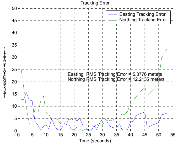
Figure 3 Box Configuration Tracking Performance For Straight Track
