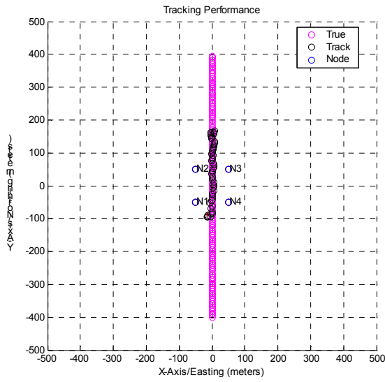
Figure 3 Box Configuration Tracking Performance For Straight Track
