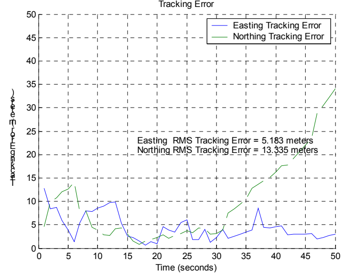
Figure 4 Diamond Configuration Tracking Performance For Straight Track
