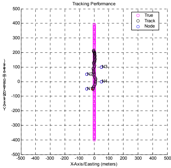
Figure 4 Diamond Configuration Tracking Performance For Straight Track
