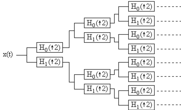
Figure 2.2 A full Tree Digital Filter Bank (DFB)
