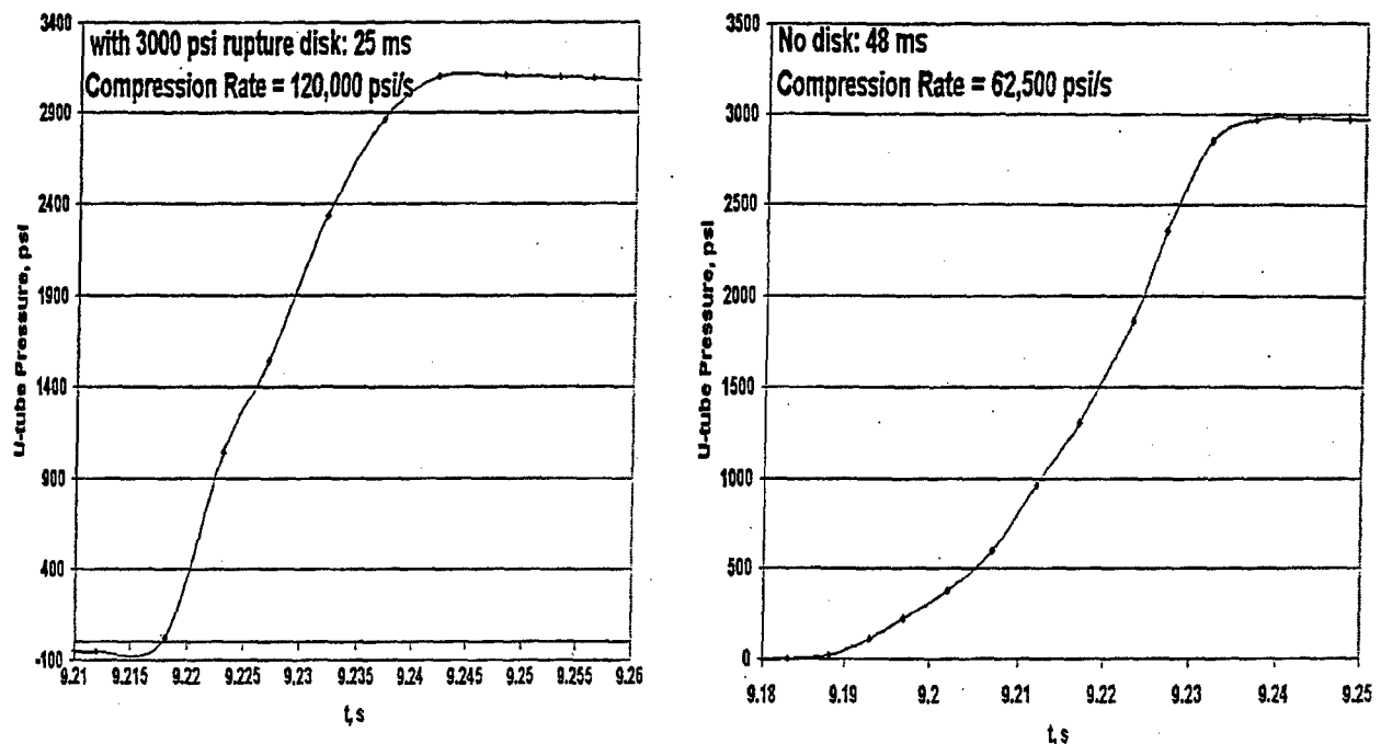
Figure 4: Compression rates of empty U-tubes with and without a rupture disk.
