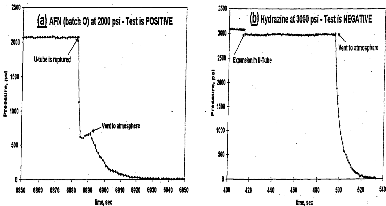
Figure 3: Typical examples of positive (a) and negative (b) compression tests.
