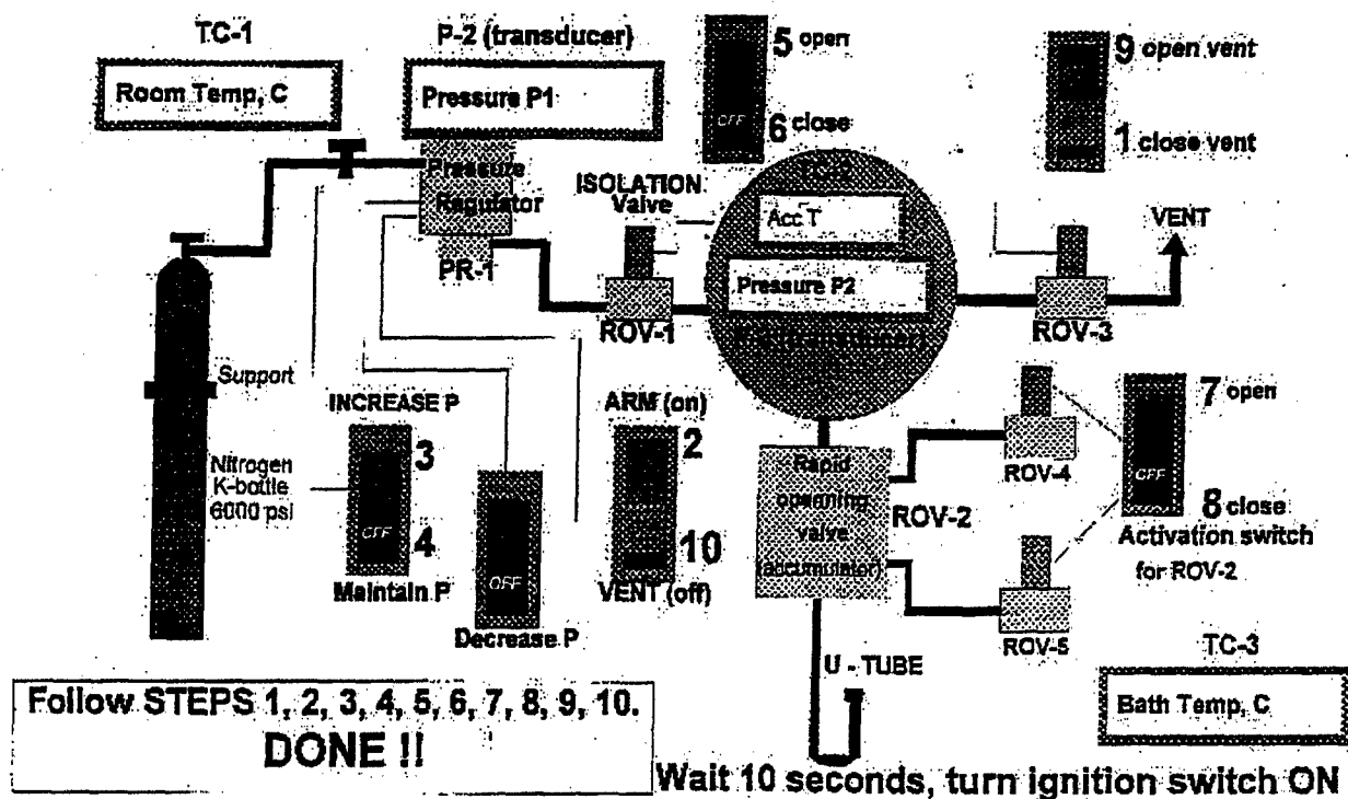
Figure 2: Control unit operating the adiabatic apparatus.
