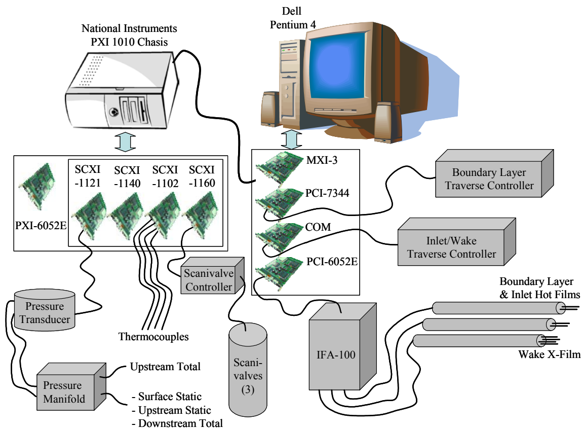
Figure 47. Instrumentation Schematic
