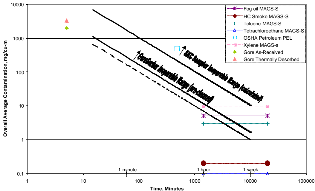
Figure 4.1 Capacity Loading Estimates for the IPCS Candidate Samplers With Selected Environmental Contaminants
