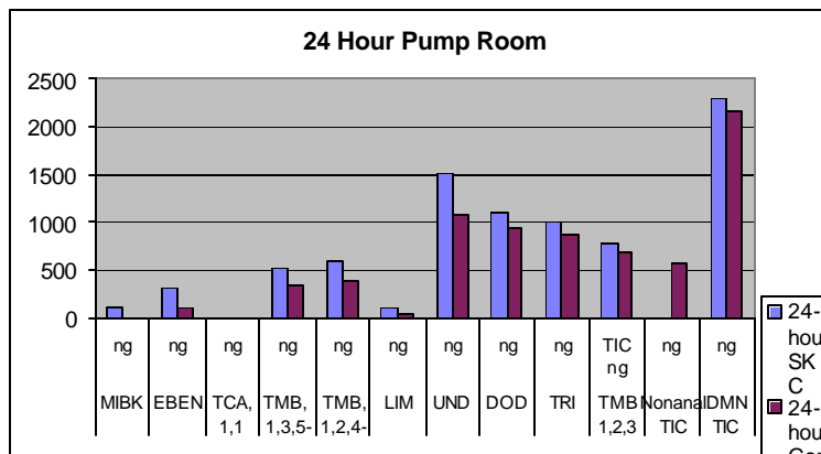
Figure 5-3. Comparison of the GoreSorbors® to the SKC Samplers for the 24-hour Sampling Period
