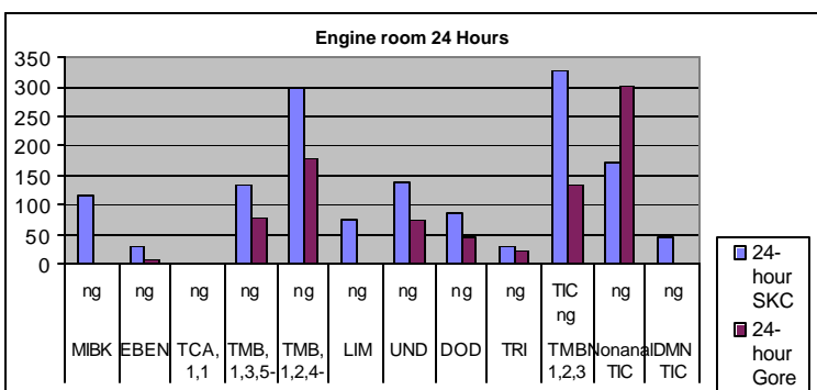
Figure 5-3. Comparison of the GoreSorbors® to the SKC Samplers for the 24-hour Sampling Period
