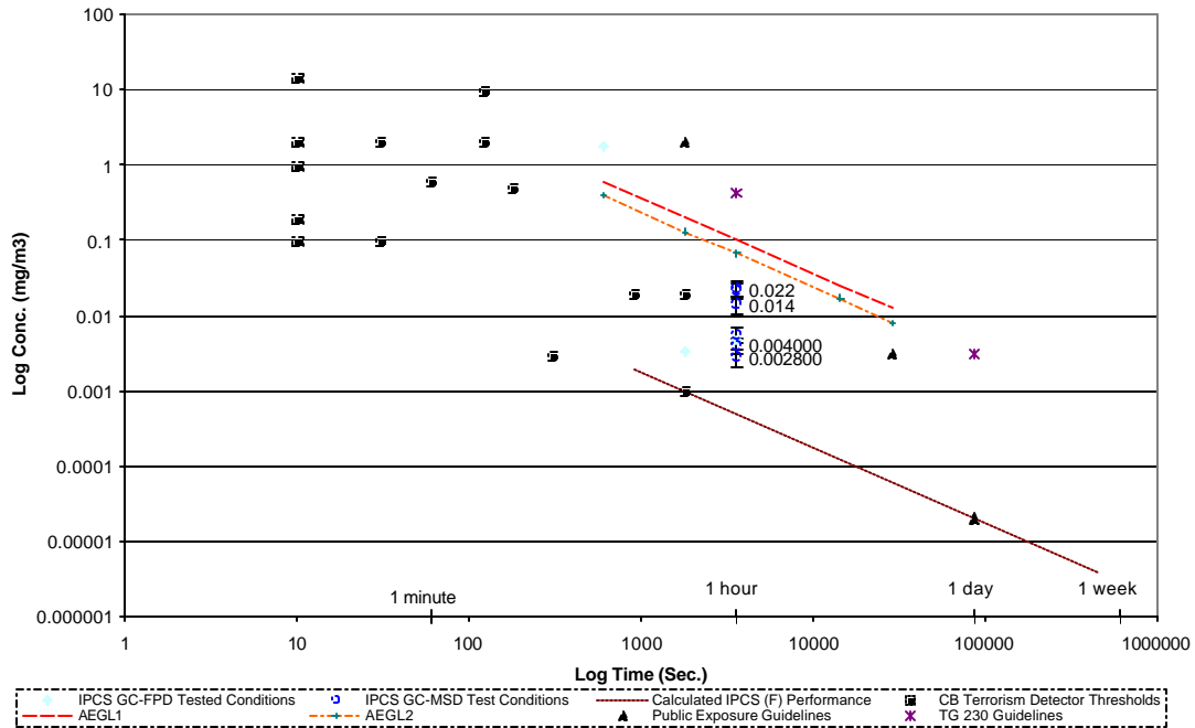
Figure 5.2 Comparison of the IPCS Detection Capability for GD to Currently Available Detectors and Exposure Guidelines
