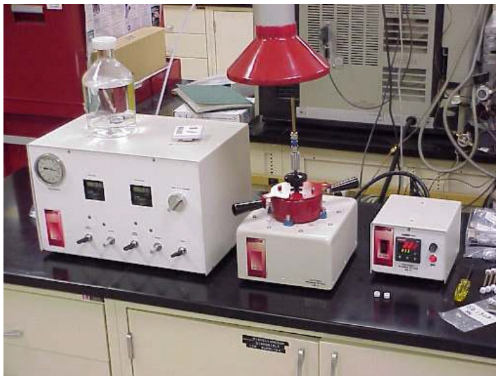
Figure 3.5 TDSorb Apparatus
