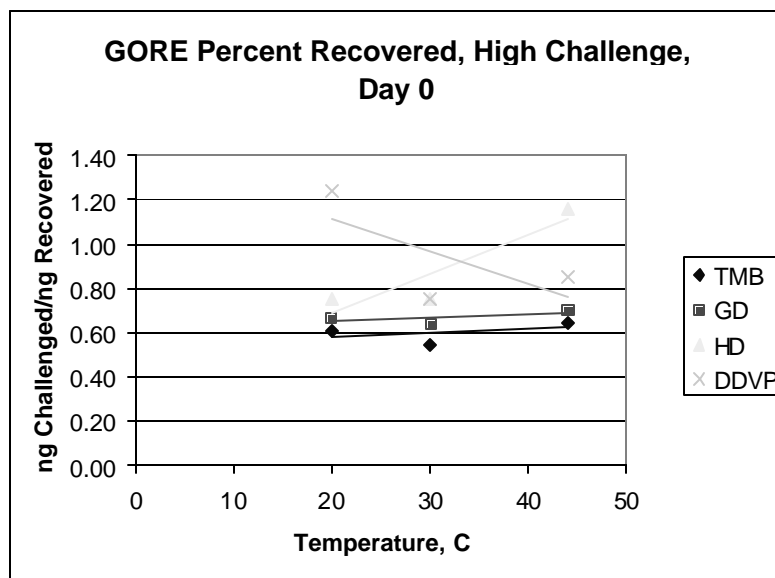
Figure 4.5 Day 0 Adsorption and Recovery Comparison Between SKC High Level and Gore High-Level Samplers
