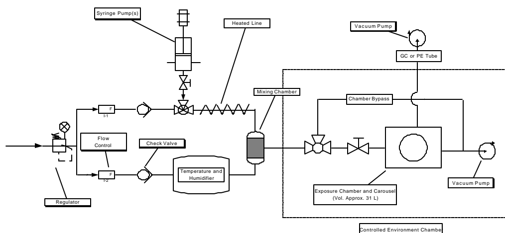
Figure 3-1 - IPCS Challenge System Schematic
