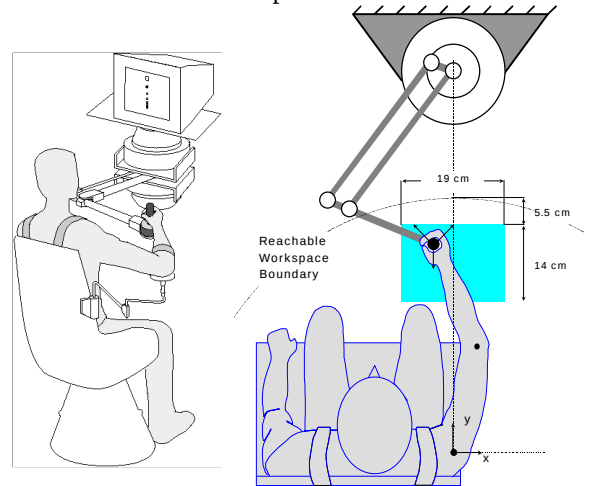
Figure 1. The subject and planar robot, driven by two brushed DC torque motors (Kolmorgen PMI JR24M4CH), controlling forces at a handle via a 4 bar linkage (Figure 1). Digital encoders (Teledyne-Gurley 25/045-NB17-TA-PPA-QAR1S) report angular position, and a force/torque sensor (ATI Gamma 30/100) reports the interface kinetics. Data were collected at 100 Hz.
