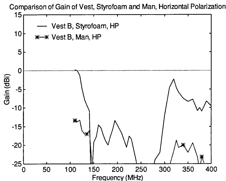
Figure 22. Boresight gain of Mark III vest on Styrofoam model and on man versus frequency. Transmitter had horizontal polarization.
