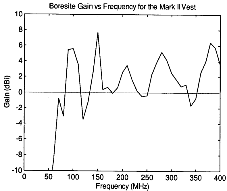
Figure 9. Boresight gain of Mark II vest antenna versus frequency between 50 and 400 MHz. A Styrofoam model supported antenna. Transmitter was vertically polarized.
