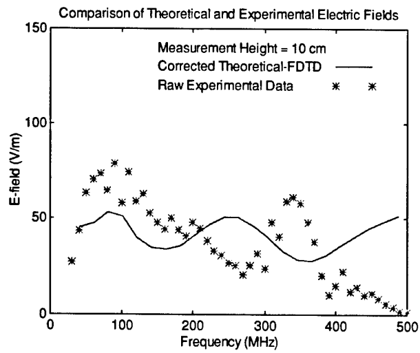
Figure 66. Comparison of theoretical with experimental results for total field versus frequency. Height of measurement is 10 cm above feed.
