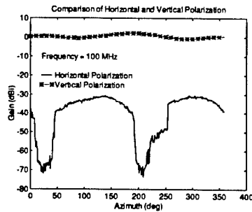
6a. Frequency = 100 MHz
