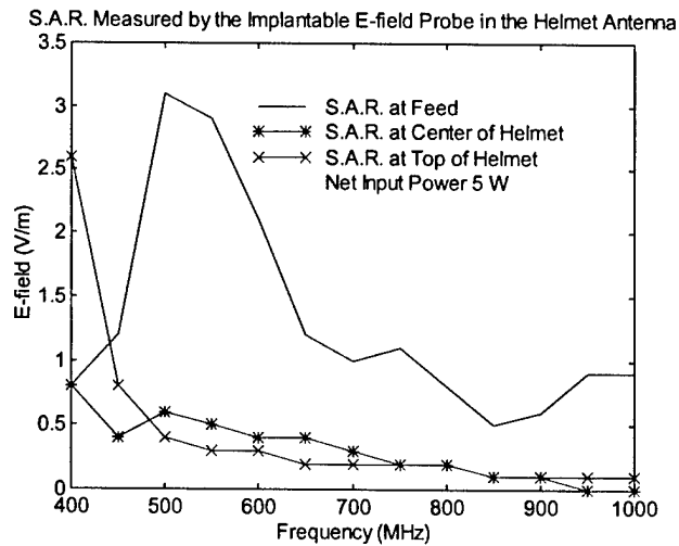
Figure 43. Measurements of specific absorption rate in W/kg versus frequency for three locations in helmet antenna.
