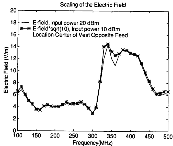
Figure 14b. Measured electric field for two values of input power. Electric field for value was multiplied by square root of 10, ratio of input powers.
