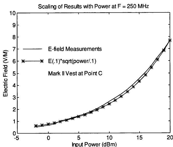
Figure 14a. Measured electric field at one frequency and many values of input power. Value of electric field for input power of 20 dBm normalized results.
