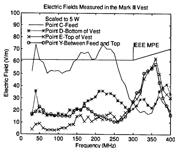
Figure 39. Electric fields measured for forward input power of 5 W. No attempt was made to measure or correct for reflected power from vest antenna.
