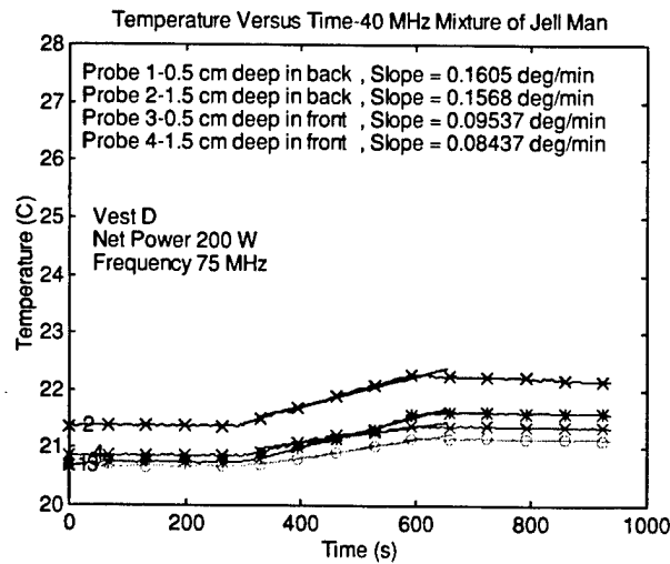
Figure 57. Temperature versus time for four probes when 200 W is input into Vest D (copper tubules behind feed and in the gap) at a frequency of 75 MHz.
