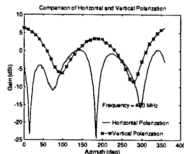
6d. Frequency = 400 MHz
