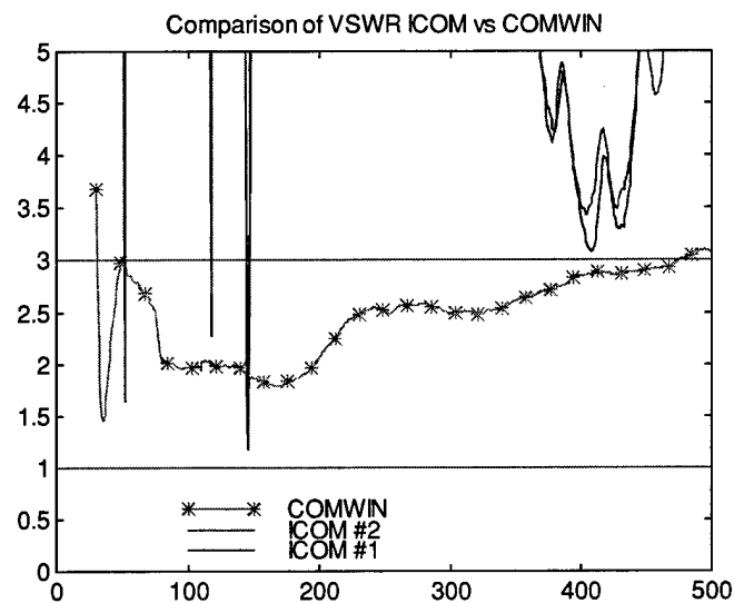
Figure 19. VSWR versus frequency of Mark III vest antenna compared with "rubber duck" antennas used for ICOM amateur band radios. ICOM antennas are excellent for four amateur bands, but unusable at other frequencies. COMWIN antenna VSWR is good at almost all frequencies between 30 and 500 MHz.
