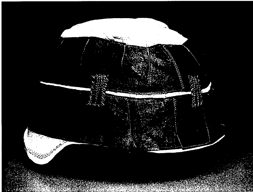
Figure 25. Mark III helmet antenna (front view)
