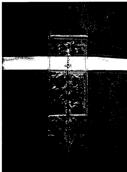
Figure 17. Close-up view of feed region of Mark III vest antenna. Capacitor with size 56 pf allowed good matching for 30- to 500-MHz frequency range.
