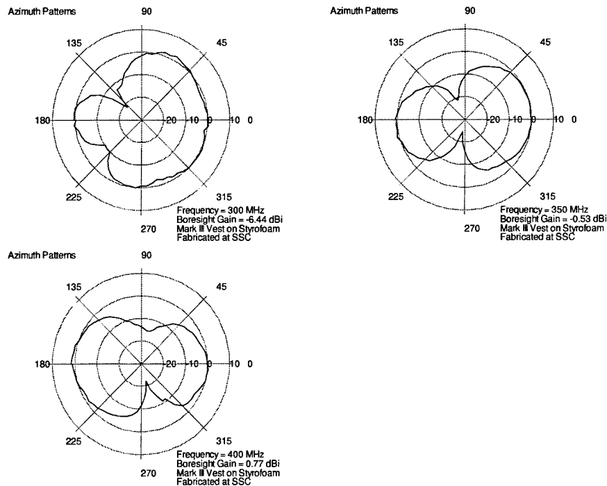
Figure 23. (continued) Radiation patterns versus azimuth angle normalized to boresight for 11 frequencies. Frequencies are 50, 125, 150, 170, 200, 225, 250, 275, 300, 350, and 400 MHz. All vest antennas become electrically large and exhibit nulls at frequencies higher than 250 MHz.
