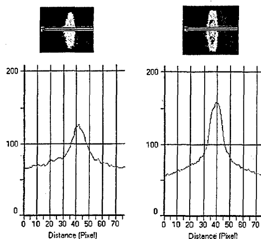
Figure 5. Averaged Raman images of LN 2 jet at sub- and super-critical chamber conditions.
