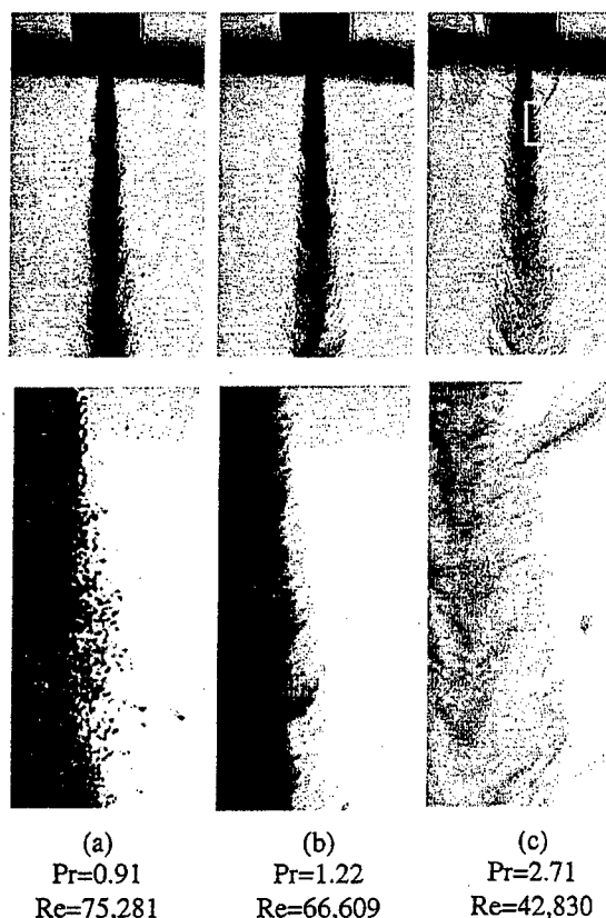
Figure 1. \text{LN}_2 injected into room temperature nitrogen at different pressures. The bottom row contains magnified images of the top row in order to examine the shear layer.
