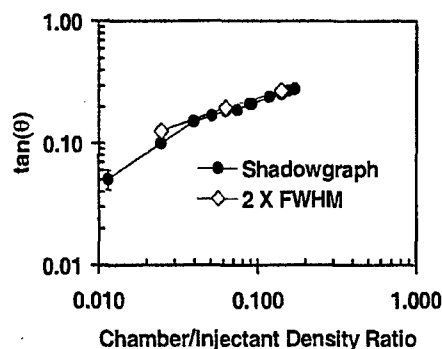
Figure 6. Comparison of the spreading angle of an N 2 /N 2 system measured using shadowgraph and spontaneous Raman techniques.
