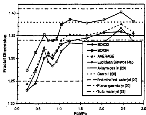
Figure 3. Fractal dimensions of the boundaries of various jets. Discrete points are data from the present effort.
