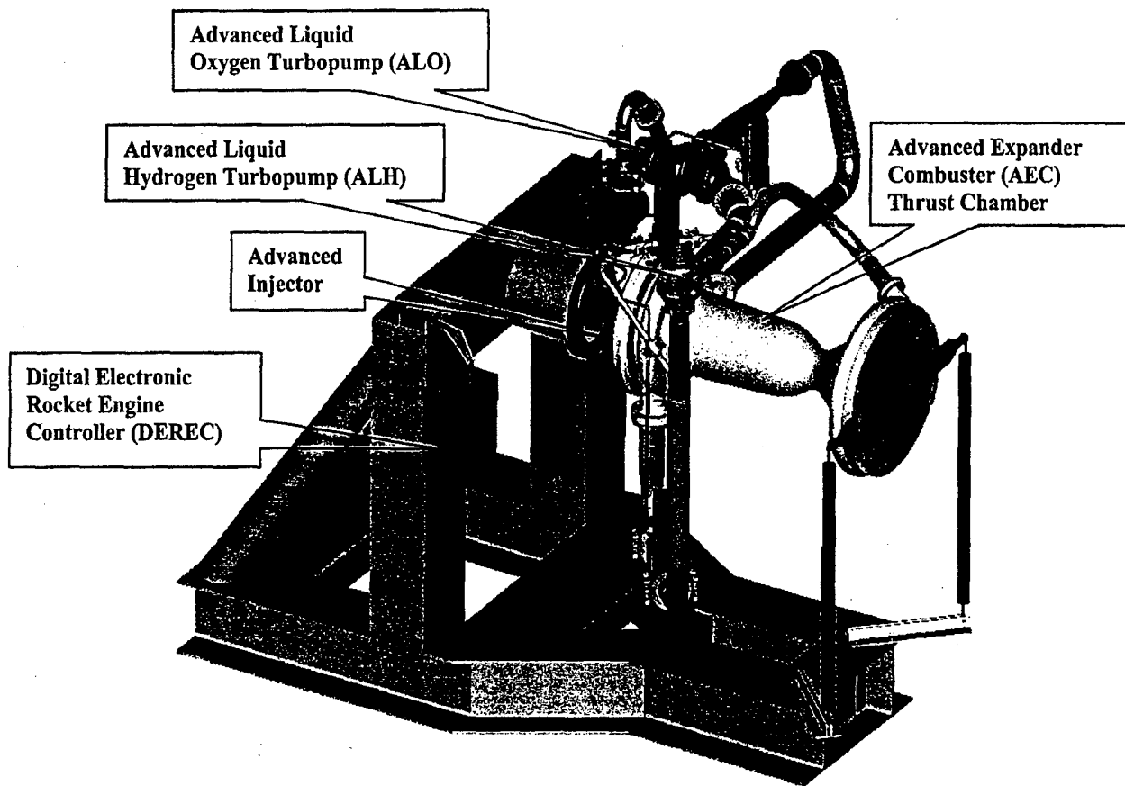
Figure 1. The IHPRPT Phase I 50k LOX/LH2 Upper Stage Demonstrator
