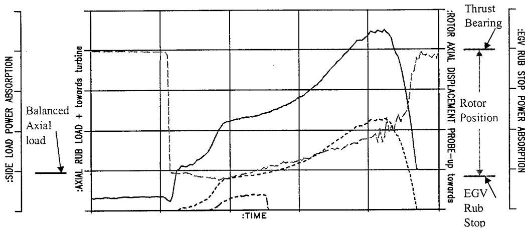
Figure 6 - Power Absorption, Axial Load Imbalance and Rotor Position for Start
