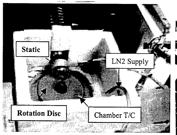
Figure 9 - Cryogenic Tribology Test Rig
