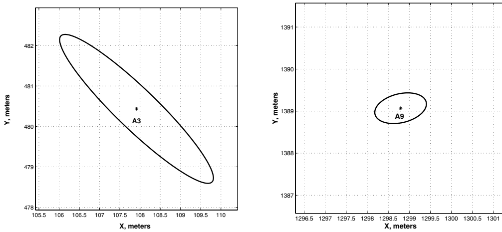
Figure 5: Two standard deviation location uncertainty ellipses for sensors A3 (left) and A9 (right) from Figure 4.
