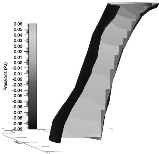
Fig. 6 : Pressure distribution along the aqueduct at about 80% of the Cardiac Cycle.
