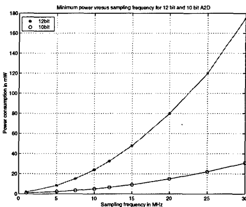
Figure 4: Minimum power for 12 bit and 10 bit ADC.
