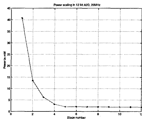
Figure 5: Power scaling for 12 bit ADC, 20MHz.
