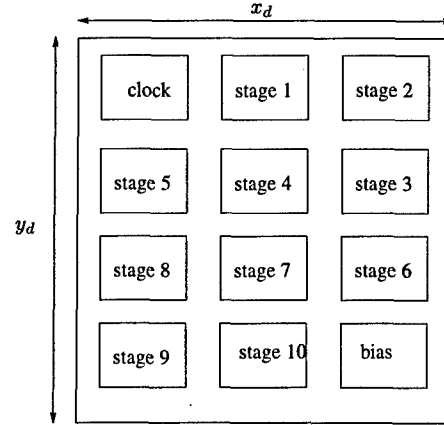
Figure 3: Floorplan of a 10 bit ADC
