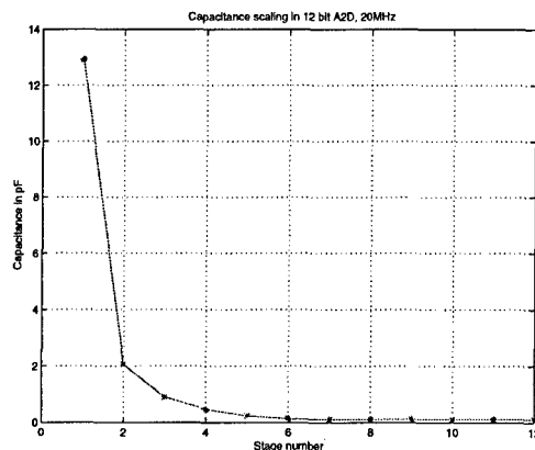
Figure 6: Capacitor scaling for 12 bit ADC, 20MHz.
