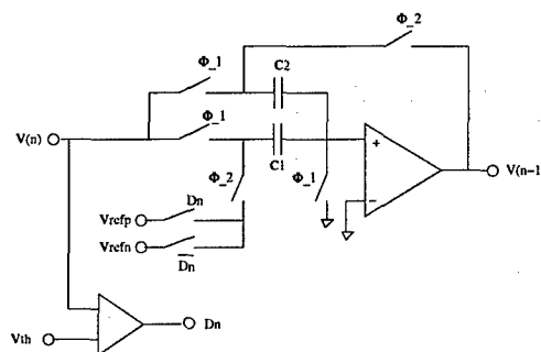
Figure 1: Single-ended implementation of a pipeline ADC stage
