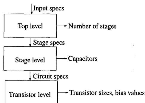
Figure 2: Hierarchical design of a pipeline ADC
