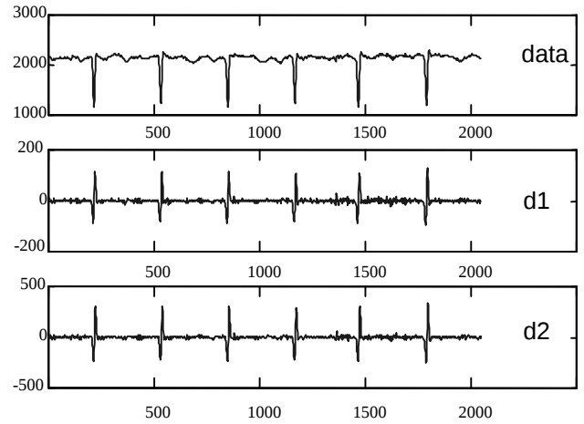
Fig. 3. Top figure shows 1-D ECG data. Middle and bottom figures show two level Dyadic Wavelet Transform, respectively. At each level, R peaks correspond to zero crossings of a minima-maxima pair in DWT with a delay of 2^{j-2} points.
