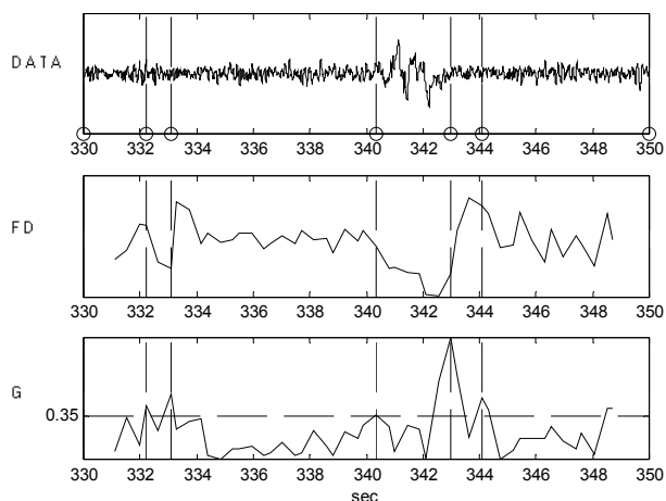
Fig. 5. Segmentation result of FD, pattern 3. Window width=1.1 sec, overlapping=60%, threshold=0.35.
