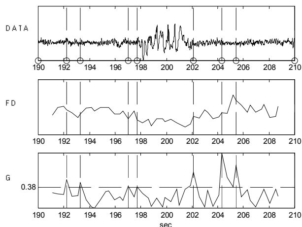
Fig. 7. Segmentation result of FD, pattern 4. Window width=1.1 sec, overlapping=60%, threshold=0.38.
