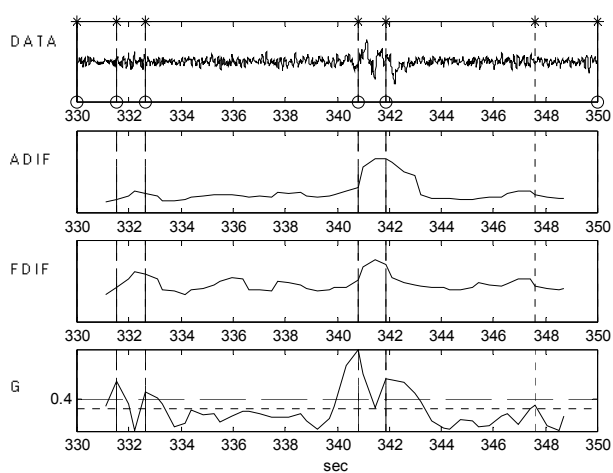
Fig. 6. Segmentation result of Värri measures, pattern 3. Window width=1.1 sec, overlapping=60%, threshold=0.3 (*) and 0.4 (o).
