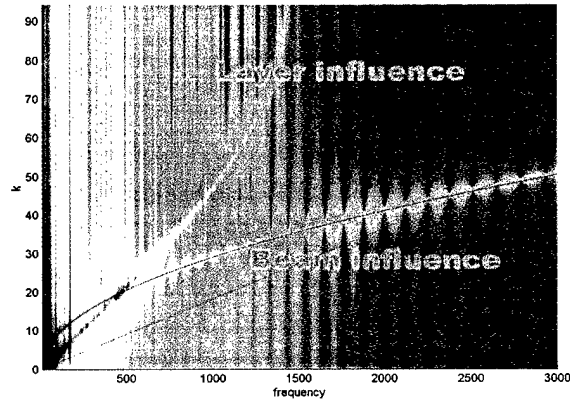
Wave Numbers in a Generic Layer
