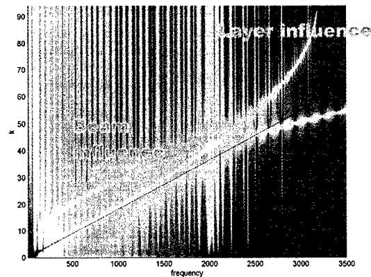
Figure 11. Dispersion plot for a tuned skin.
