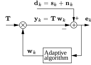
Fig. 1. Adaptive block-wise estimation of truncated expansions.
