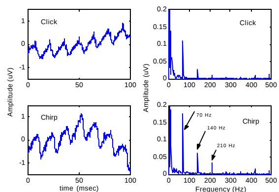
Fig. 2 Sample ASSR recordings from a subject in the time domain (left) and the frequency domain (right). The click (top) and chirp (bottom) stimuli were both presented at 70 Hz repetition rate. In addition to the main frequency component at 70 Hz, the second and third harmonics are also observed.
