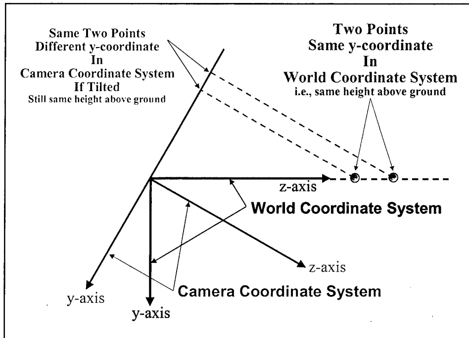
Figure 8. Effect on y-coordinate because of tilted coordinate system.
