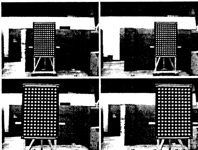
Figure 3. Left camera images of the calibration poster, clockwise, left rear, right rear, right front, and left front.
