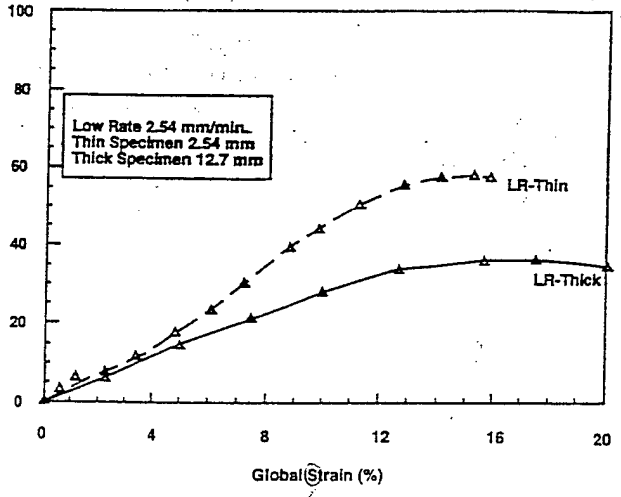
Fig. 2 Load-strain relations ( T=73.9^{\circ}\text{C} )
