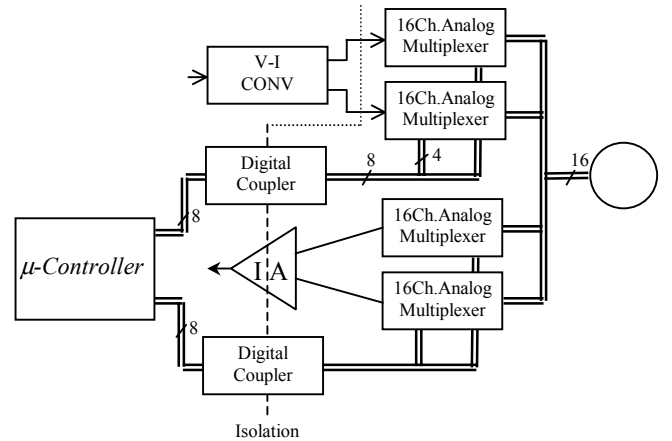
Fig. 4. Multiplexer and demultiplexer part
