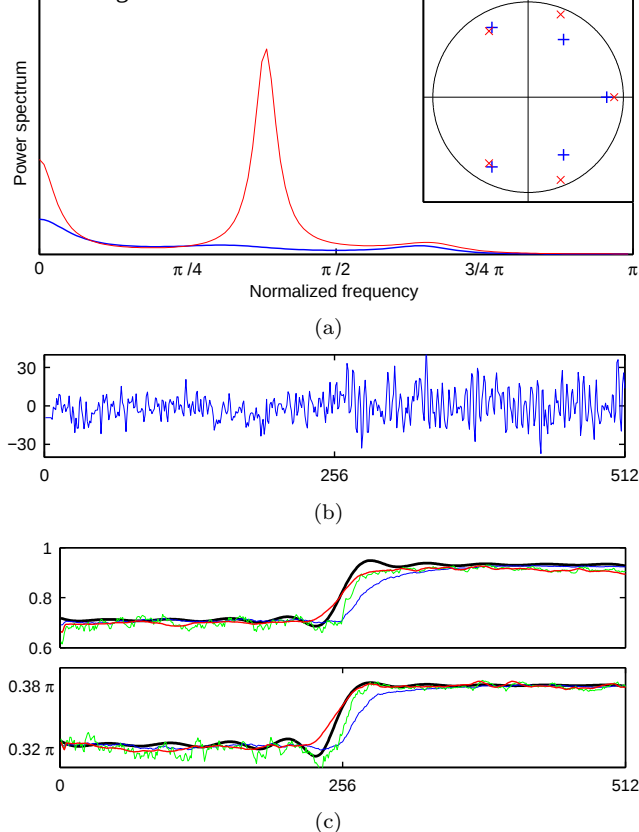
Fig. 2. A realistic simulation of EEG transition as an AR(5) process. (a) The roots and the corresponding spectra before (blue) and after (red) the transition. (b) A typical realization of the process. Averaged estimates over 100 realizations of the modulus and phase angle of the root corresponding to alpha activity are presented in (c), where true values (black), Kalman smoother estimates (red) and RLS estimates (blue/green) are shown. The state noise covariance coefficient of the Kalman smoother was \sigma_w^2 = 8 \cdot 10^{-5} and the forgetting factors of RLS were \lambda_1 = 0.98 (blue) and \lambda_2 = 0.9 (green).
