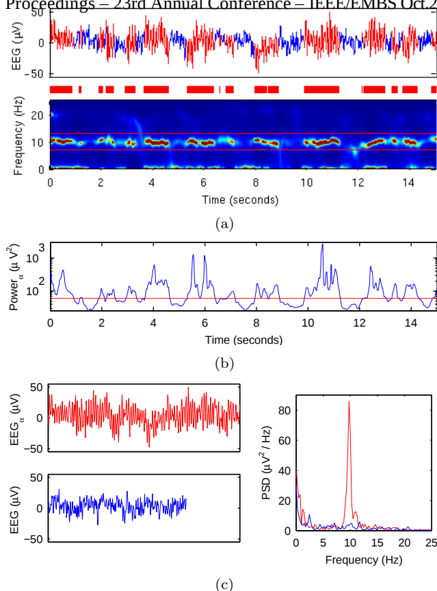
Fig. 4. Kalman smoother applied to alpha rhythm detection. (a) An EEG sample of 15 seconds from channel O2 measured from subject having eyes closed and the corresponding time-varying PSD. (b) Detection is based on thresholding the power integral over the alpha band (7–13 Hz) with a threshold of 10 \mu V^2/Hz . Block (c) presents PSD estimates (calculated with traditional FFT based method) for the signals obtained by concatenating the EEG epochs where alpha activity was detected (red) or not detected (blue).
