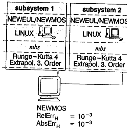
Figure 9: Simulation parameters and setup
