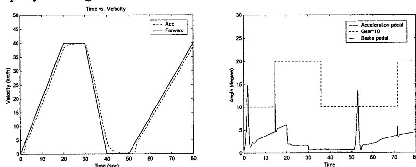
Figure 6. Stop-and-go Simulation
