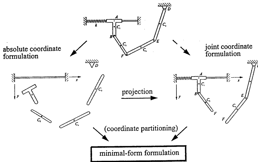
Fig. 3. Treatment of closed-loop systems.
