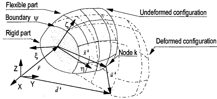
Figure 6. Flexible body with a rigid part
