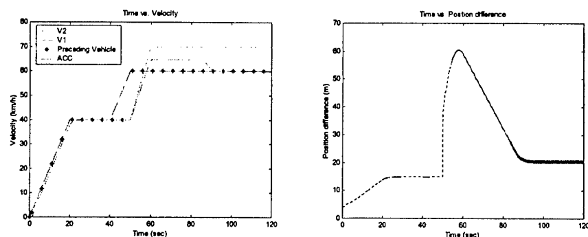
Figure 7. Cut-out simulation
