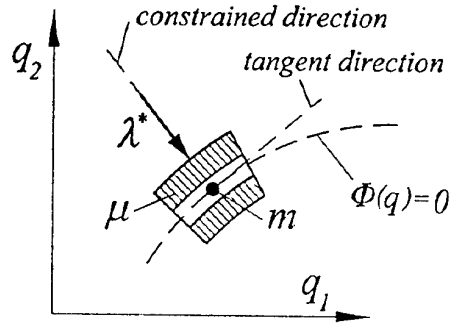
Fig. 5.. The geometric interpretation of the augmented Lagrangian formulation.
