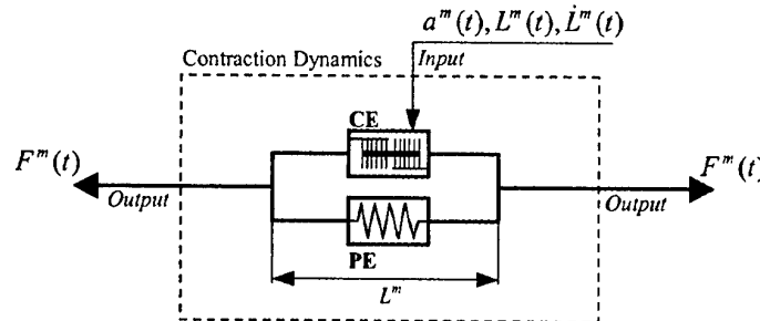
Figure 5. Contraction dynamics using a Hill-type muscle model.
