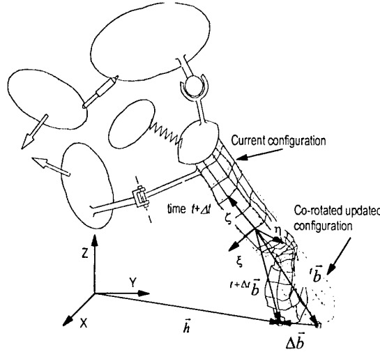
Figure 1. Generic multibody system in an impact fictitious scenario
