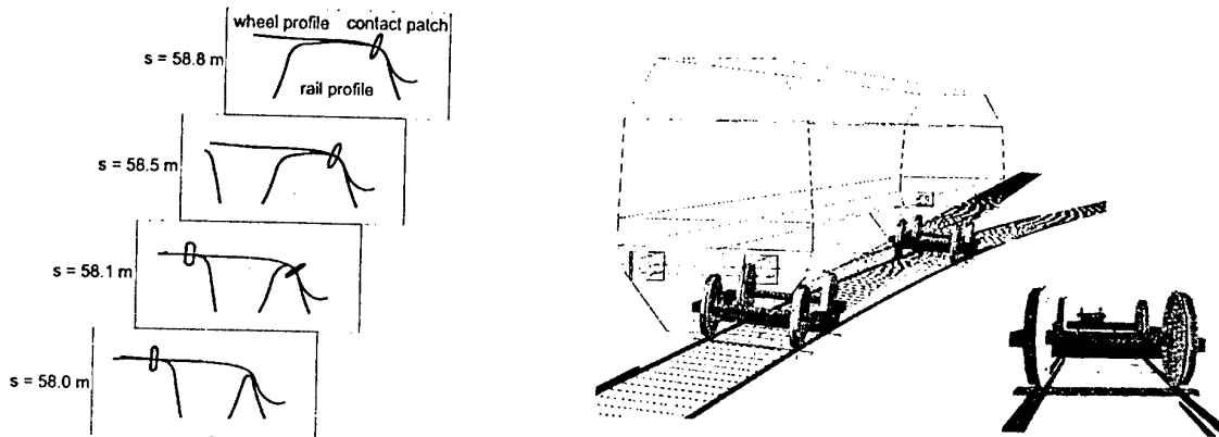
Figure 4. Passenger car running through a switch. Left: Contact patches between left wheel and running rail in the vicinity of the crossing vee. Right: Snap-shot of simulation model with leading bogie entering the common crossing and the inner wheels being guided by the check rail (large - back view, small - front view).
