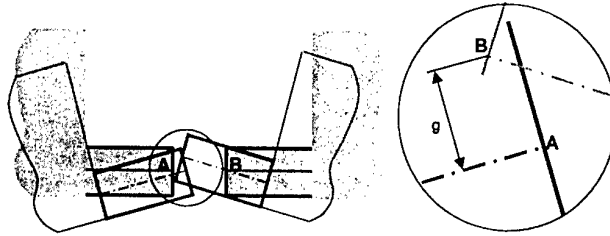
Figure 12. Anti-climber device contact geometry
