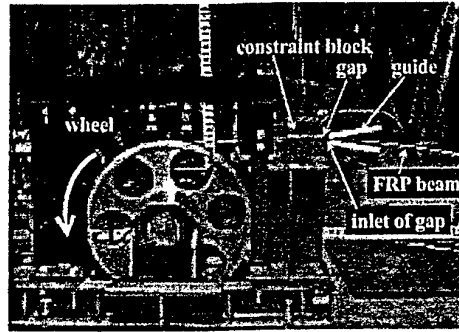
Fig.4 Experimental setup
