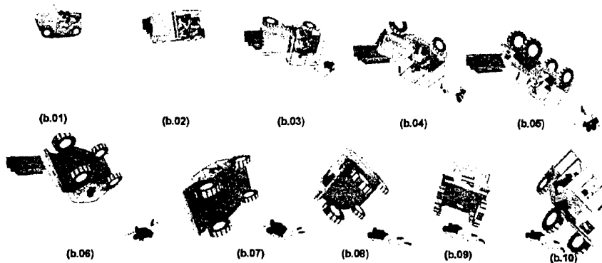
Figure 27. Front view of the rollover simulation of a vehicle with three occupants
