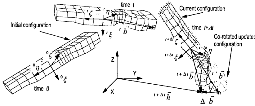
Figure 5. General motion of a flexible body
