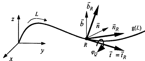
Figure 4 – Cant angle contribution to the track model
