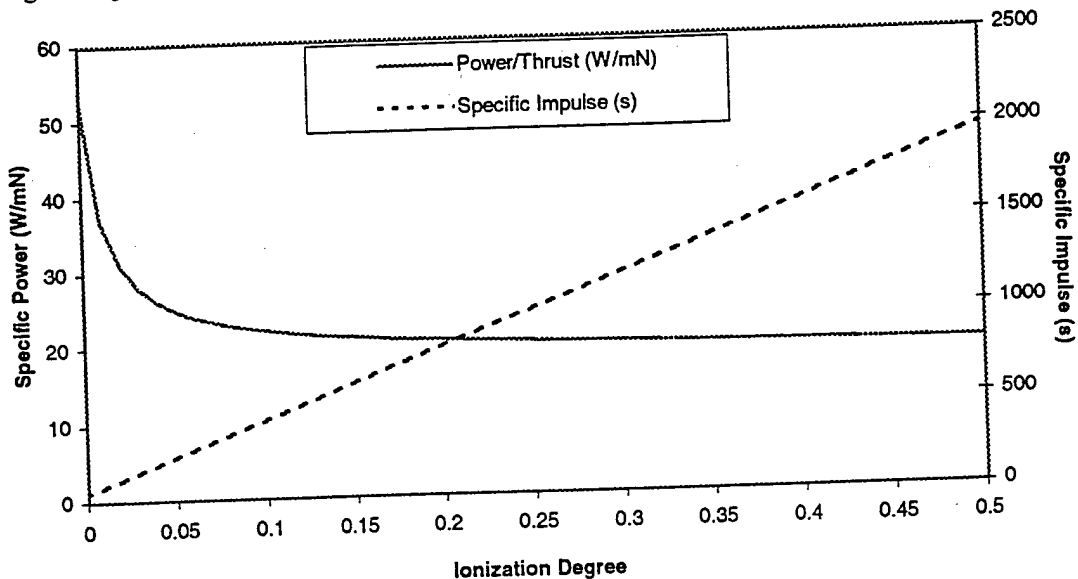
Fig. 1 Effect of ionization degree on performance of NMIMT with typical discharge chamber
