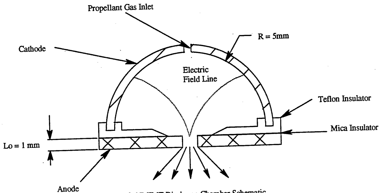
Fig. 2 NMIMT Discharge Chamber Schematic
