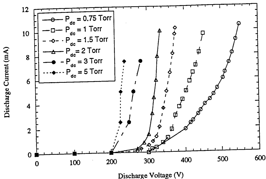
Fig. 5 V-I Characteristics of the NMIMT Discharge Chamber
