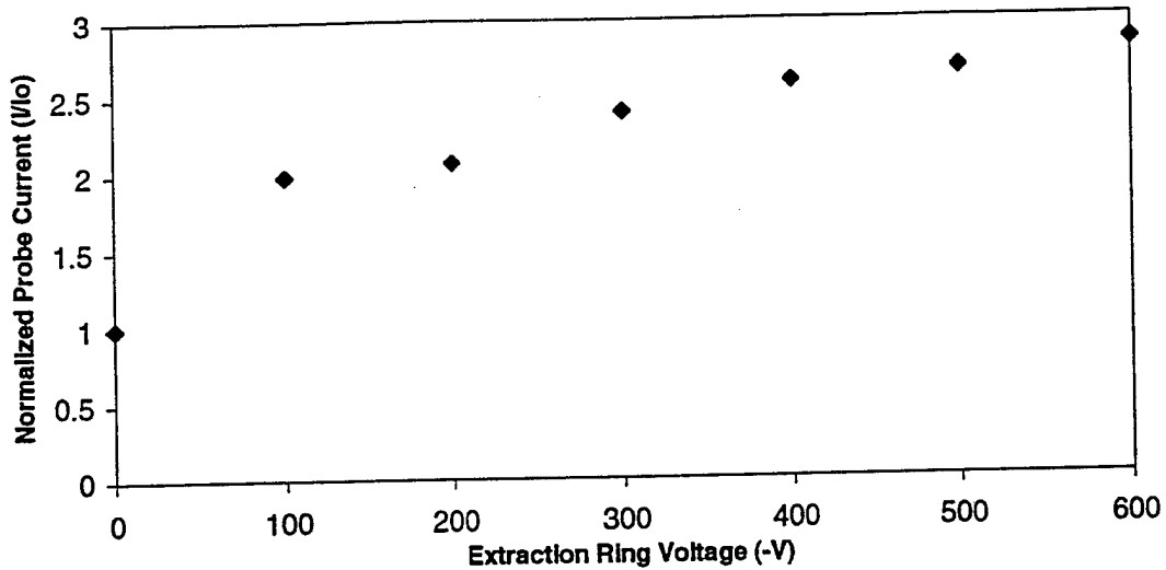
Fig. 10 Extraction Ring Effect on Discharge Chamber Plume
