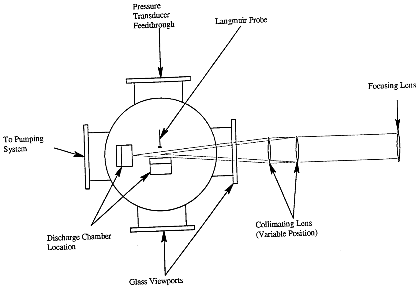
Fig. 4 Diagnostics Setup
