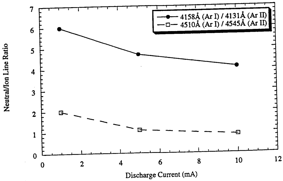
Fig. 7 Neutral to Ion Ratios at Different Discharge Conditions
