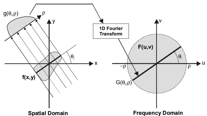
Fig 4. The Fourier Slice Theorem.
