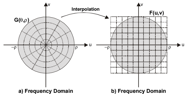
Fig. 5. Interpolation in frequency domain.
