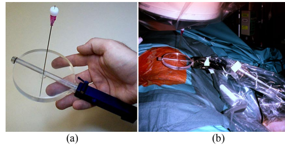
Figure 1. The PAKY needle driver. (a) Close-up. (b) Used surgically for image-guided percutaneous renal access.
