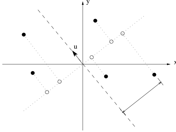
Figure 1: Geometrical interpretation of G(B, \phi) as the sample variance of the array locations projected onto the line orthogonal to u
