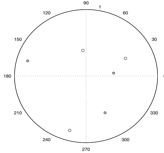
Figure 3: A 6 element isotropic array (circles and stars) formed from rotating a randomly generated 3-element subarray (stars) by 90^\circ .
