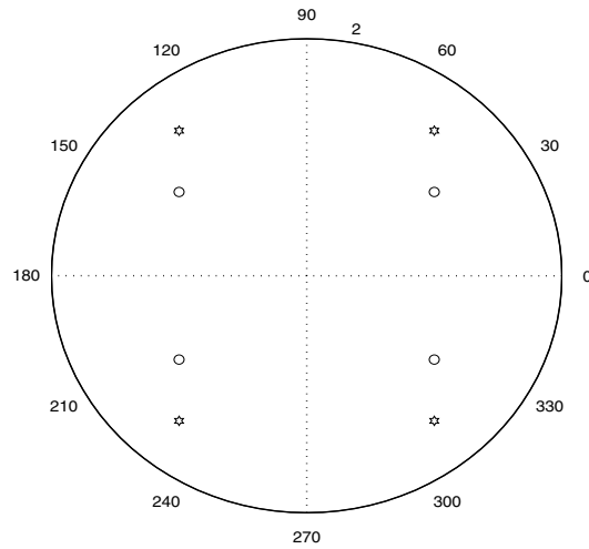
Figure 5: An 8-element isotropic array formed by combining two X-shaped geometries.
