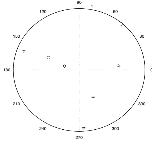
Figure 4: A 7-element isotropic array formed from an arbitrary 5-element subarray (stars) by adding 2 elements (circles).
