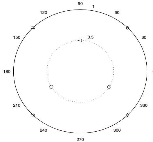
Figure 2: An isotropic planar array obtained as the superposition of a 4 element and a 3 element circularly symmetric array.
