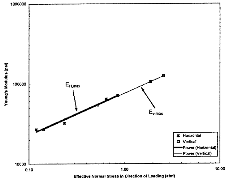
Figure 8.13 E_{V,max} and E_{H,max} vs. the effective normal stresses in direction of loading for Site 5
