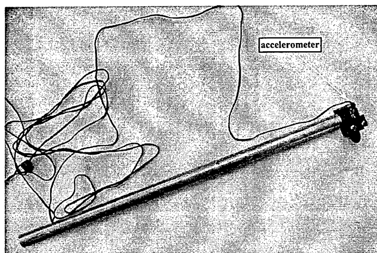
Figure 5.16 Source hammer and accelerometer
