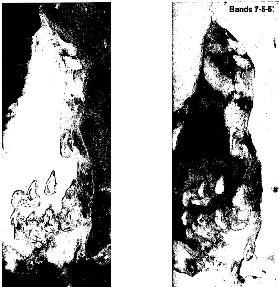
Figure 7. Multispectral images of Lake Frome, South Australia. The spectral bands represented by red, green, and blue, respectively, are indicated at the top of each image
